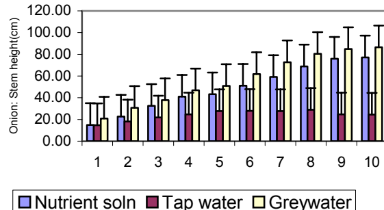
Figure 2: Stem height of green pepper (A), spinach (B), beetroot (C) and onion (D), monitored throughout the second trial crop cycle. Figures show means for 15 plants.
