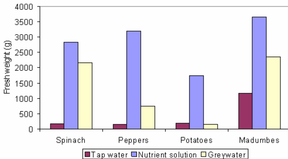
Figure 3. Total yield for spinach, green peppers, potatoes and madumbes for one crop cycle. This figure shows a total yield measured in fresh weight for all plants
