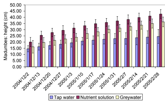
Figure 1: Stem height of spinach (A), green peppers (B), potatoes (C) and madumbes (D), monitored throughout one crop cycle. Figures show means and standard deviations for 25 plants.
