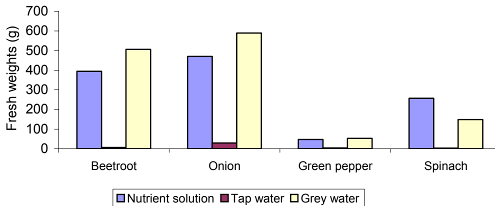
Figure 4: Total yield over time for beetroot, onion, green pepper and spinach. This figure shows a total yield measured in fresh weight for all plants.
