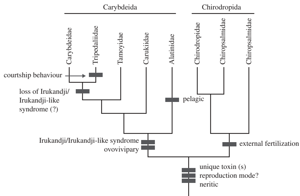
Figure 3. Trends in toxicity and life-history evolution; phylogenetic relationships follow figure 1.
