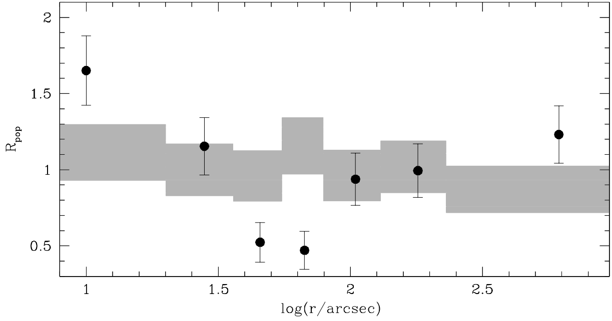
Fig. 8.— Double normalized ratio (see text) of BSSs (dots and error bars) and of HB stars (gray regions).
