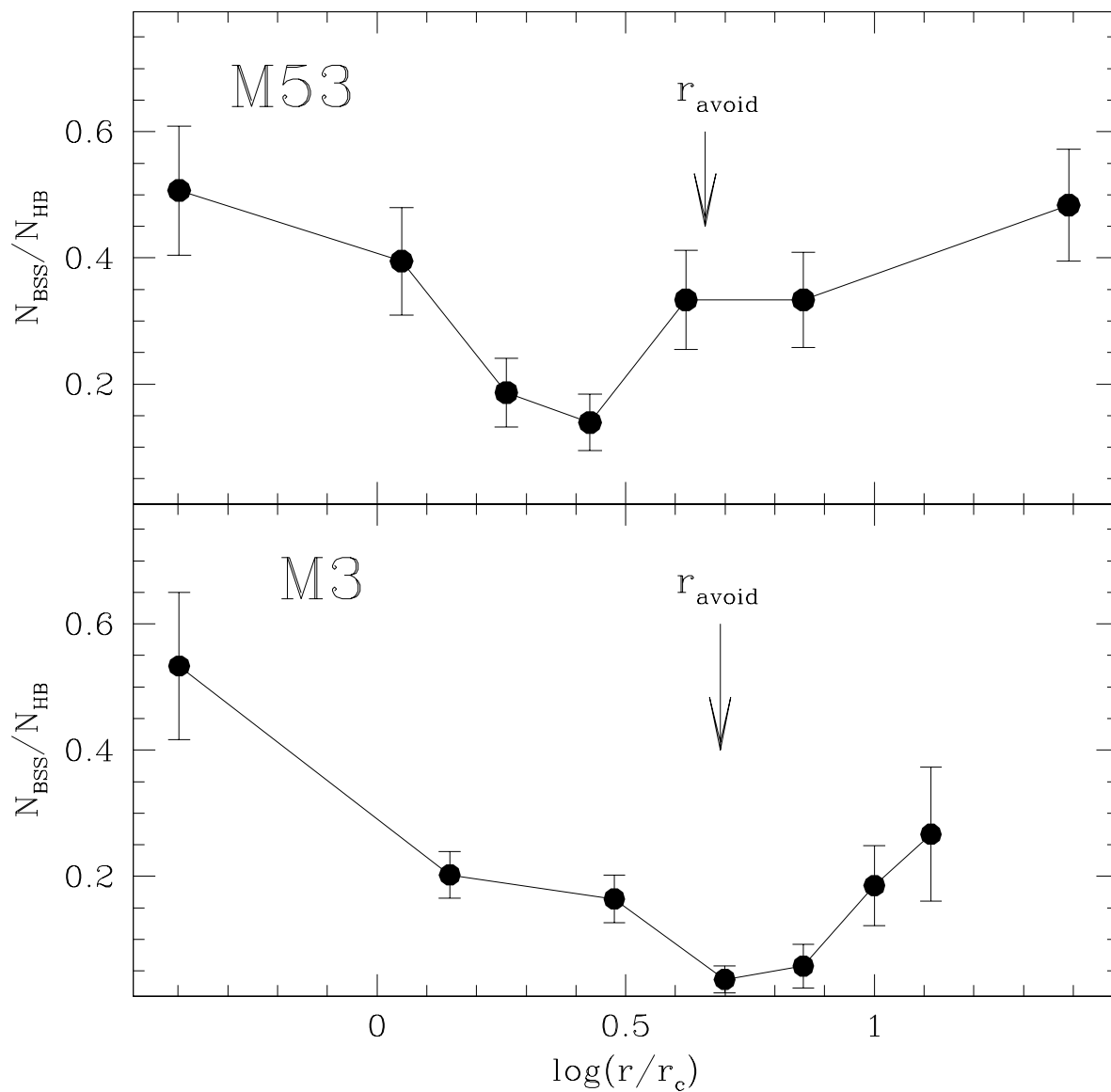
Fig. 9.— Relative frequency of BSSs with respect to HB stars for M53 ( upper panel ) and M3 ( lower panel ), plotted as a function of the distance from the cluster center in units of r_c . Vertical arrows mark the estimated position of the radius of avoidance of the two clusters (see text for details).
