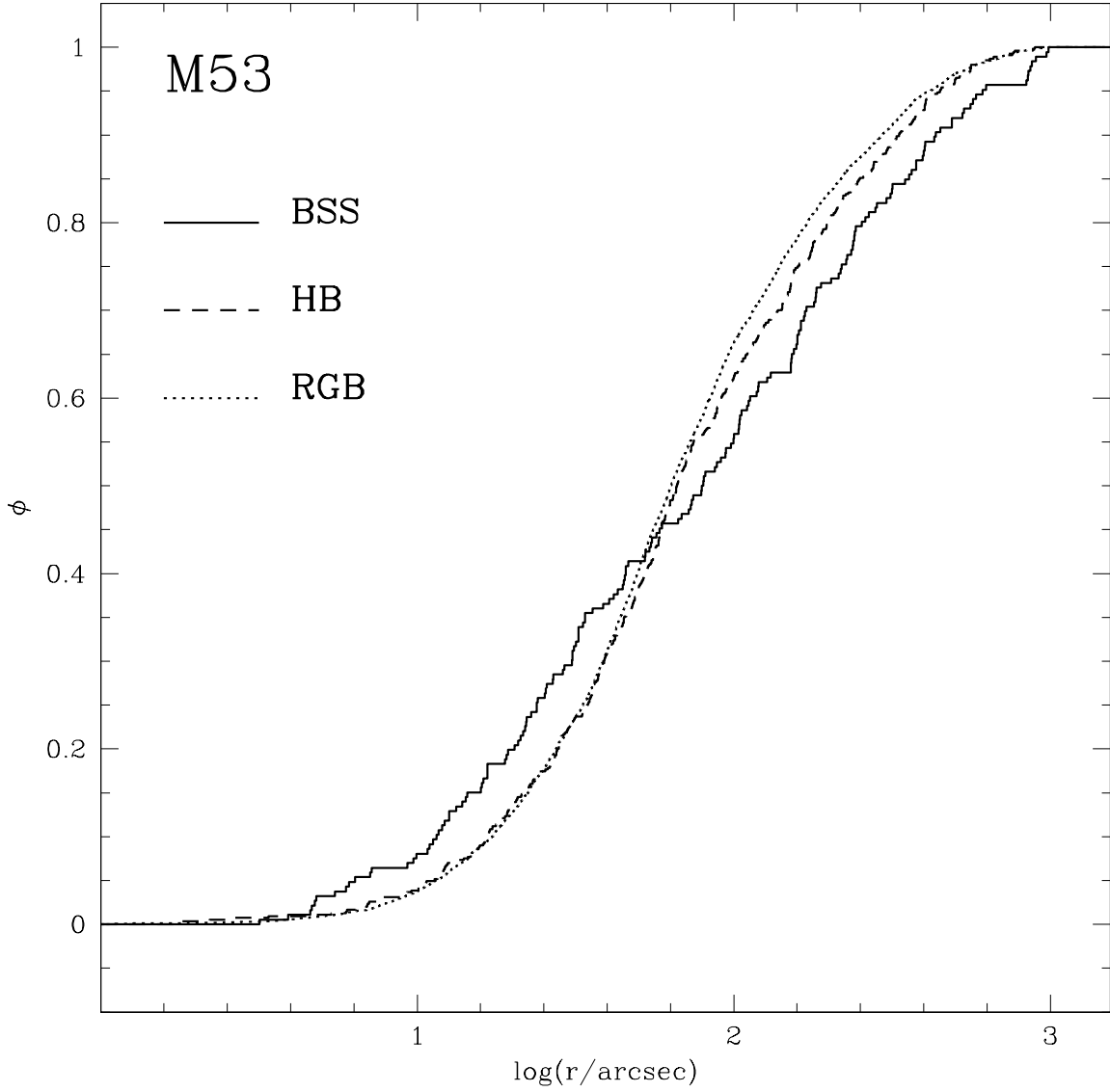
Fig. 6.— Cumulative radial distribution of BSSs ( solid line ), HB stars ( dashed line ) and RGB+SGB stars ( dotted line ), as a function of the projected distance from the cluster center.
