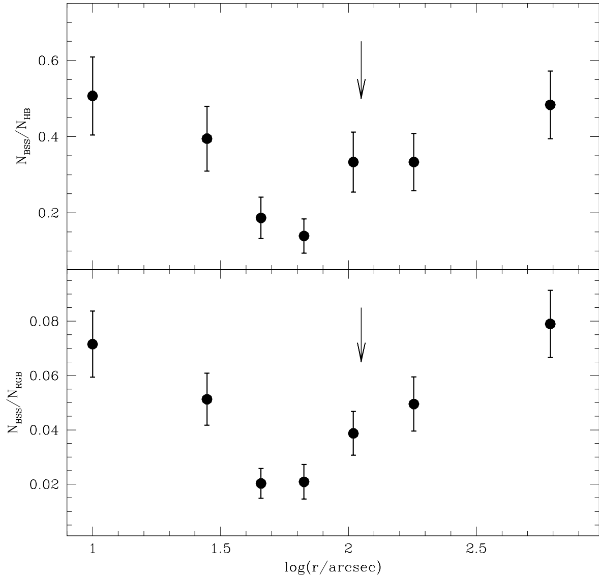
Fig. 7.— Relative frequency of BSSs with respect to HB ( upper panel ) and RGB+SGB stars ( lower panel ), plotted as a function of the distance from the cluster center. The vertical arrows represent the estimated position of the radius of avoidance of the cluster (see text for details).
