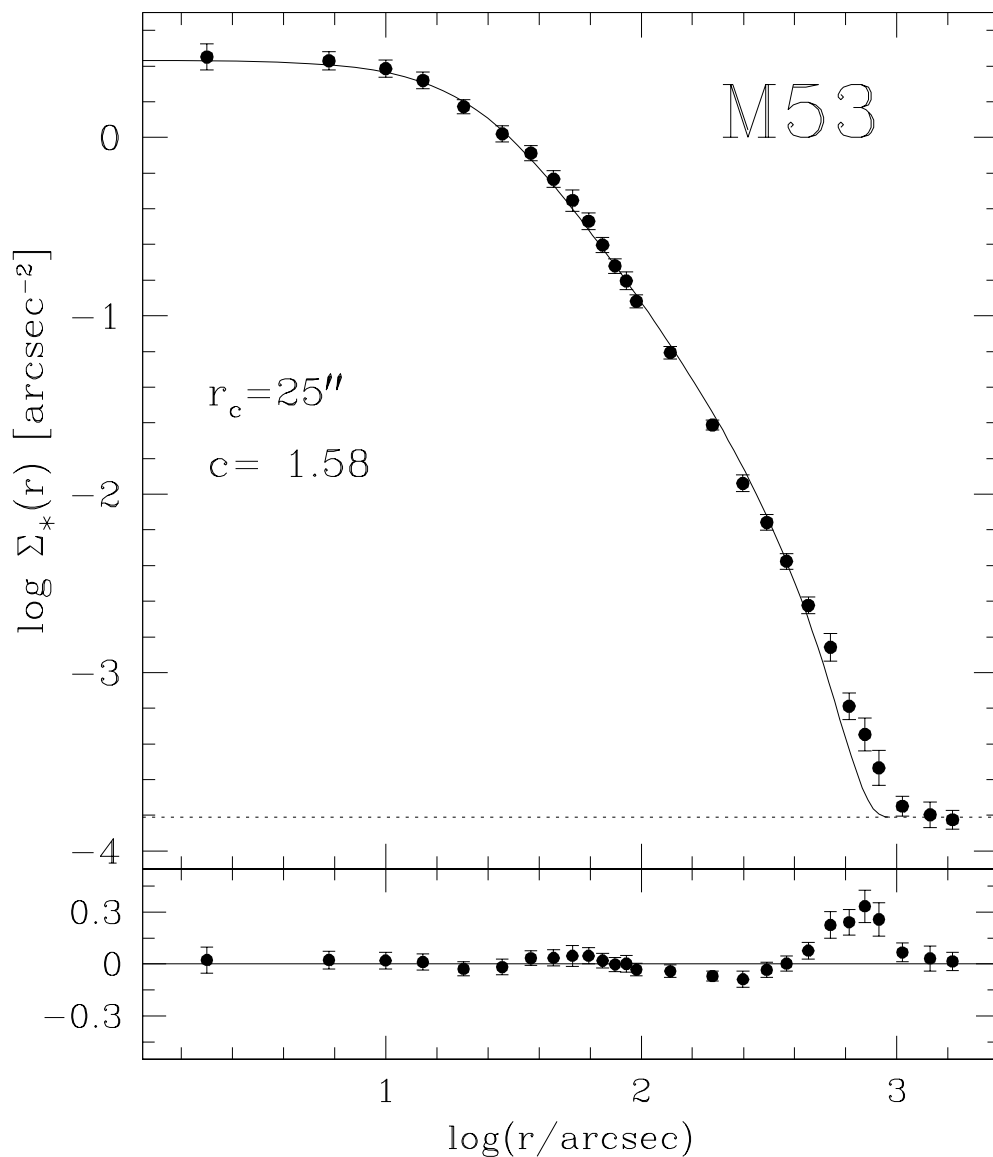
Fig. 4.— Observed surface density profile (filled circles and error bars) in units of number of stars per square arcseconds. The solid line is the King model ( c = 1.58 ; r_c = 25'' ) that best fits the observed density profile over the entire cluster extension. A value of 0.54 \text{ stars/arcmin}^2 is adopted as the field contamination density (dashed line). Notice that starting from a radius r \gtrsim 16.6' field star counts become dominant.
