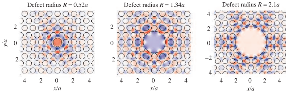
Figure 3: Accelerating modes of several photonic crystal fiber configurations. The shading indicates the axial electric field, which is also the direction of propagation of the mode.
