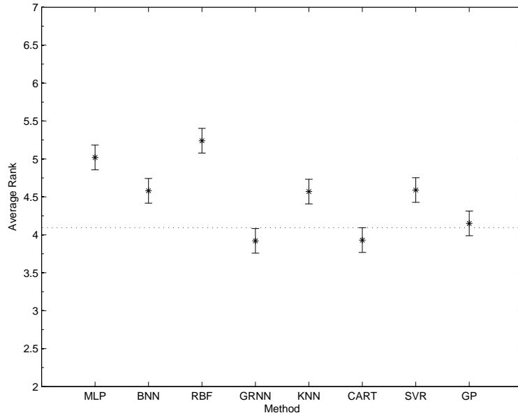
Figure 2: The average ranks with 95% confidence limits for the multiple comparison with the best test for the DIFF preprocessing method. The dashed line indicates that any method with confidence interval above this line is significantly worse than the best (as described in Section 5 immediately before Eq. (22)).
