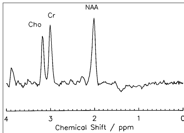
Fig 2. A control cerebellum spectrum obtained with a spin-echo sequence (1600/135/256) and a voxel size of 2 \times 2 \times 2 cm 3 .
