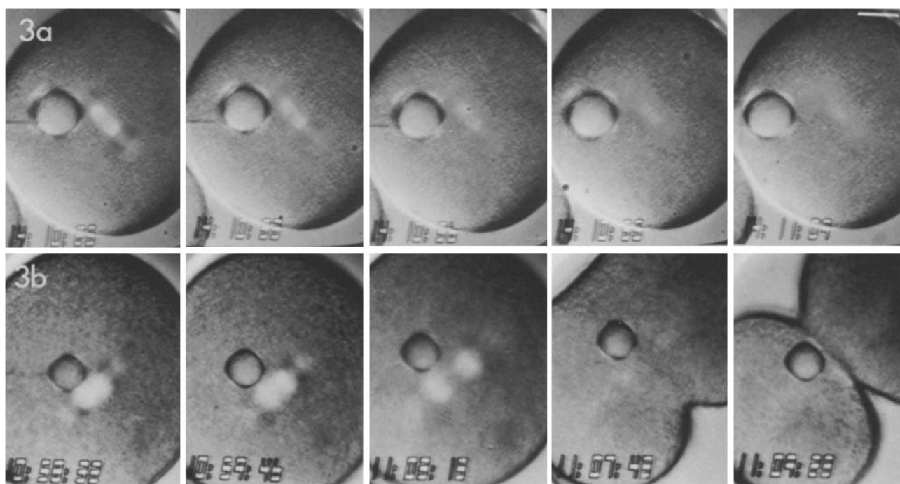
FIGURE 3 Video records of the response of spindle assembly, seen with polarization microscopy, to microinjection of intracellular concentrations of (a) 1.5 mM colchicine into a first-division metaphase embryo (b) and 0.75 mM lumicolchicine into a first-division metaphase embryo. Time in hours:minutes:seconds is given on each frame by the video time-date generator. In a note that most of the half-spindle and astral BR disappears in 20–25 s after injection. The BR remaining after 20–25 s corresponds to differentially stable kinetochore fiber microtubules (see text). Note that lumicolchicine has no effect on spindle assembly or cell division (b). Photographs were made from the video monitor. Bar, 30 \mu\text{m} . \times 270 .
