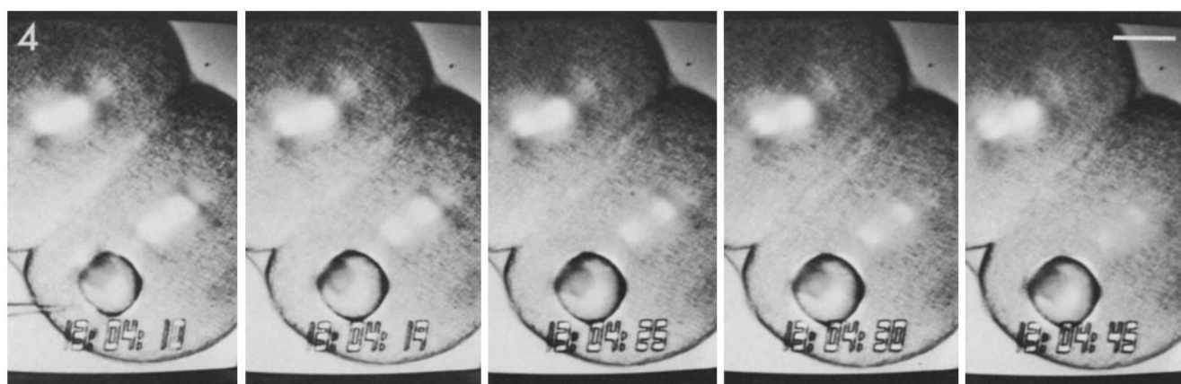
FIGURE 4 Microinjection of 0.75 mM intracellular concentration of colchicine into one cell of a second division, mid-anaphase embryo. Observations were recorded as described in the legend of Fig. 3. Like metaphase spindles, most of the half-spindle and astral BR disappears in 20–25 s after injection; only the differentially stable kinetochore fiber BR remains (see text). Note that the spindle in the noninjected cell is unaffected by colchicine injection into the neighboring cell. Bar, 30 \mu\text{m} . \times 300 .
