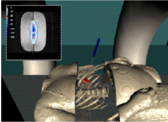
Figure 3. Output visualization of the VERTEX system while providing support for a (simulated) cryosurgery. The trunk of the patient is shown in the workspace of an open-field NMR machine. The segmented liver tumor has been extracted from previous NMR scans and is visible in real time but with reduced resolution in the operating room. Also shown is the location and orientation of the cryogenic probe being positioned by the surgeon. The visible insert shows the shape of the corresponding cold front predicted from a finite-element simulation of heat transfer in the tissue.
