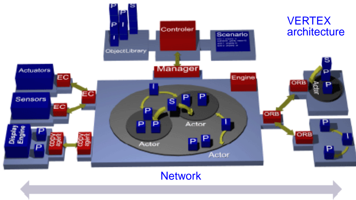
Figure 2: The VERTEX architecture is net-centric and consists of modules which are interconnected through a CORBA-based software bus implemented on a high-speed network with Quality of Service capabilities. The simulation kernel, shown in the center and right-hand side, forms the core of the system, and integrates actors, properties and interaction in an object-oriented framework. User interfacing, shown on the left-hand side, is not part of the critical simulation loop, which executes on a hard real-time OS within the kernel. Other supporting components such as the object library, overall control and scenario editing support, are shown in the background.
