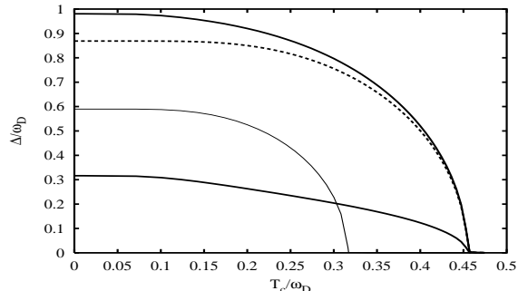
FIG. 2. Superconducting order parameters \Delta_i in the multi-gap weak-coupling approximation (solid lines), and in the isotropic (dirty) BCS limit (thin line). The BCS order parameter corresponding to the the same T_c as the multigap model is shown by the dashed line.
