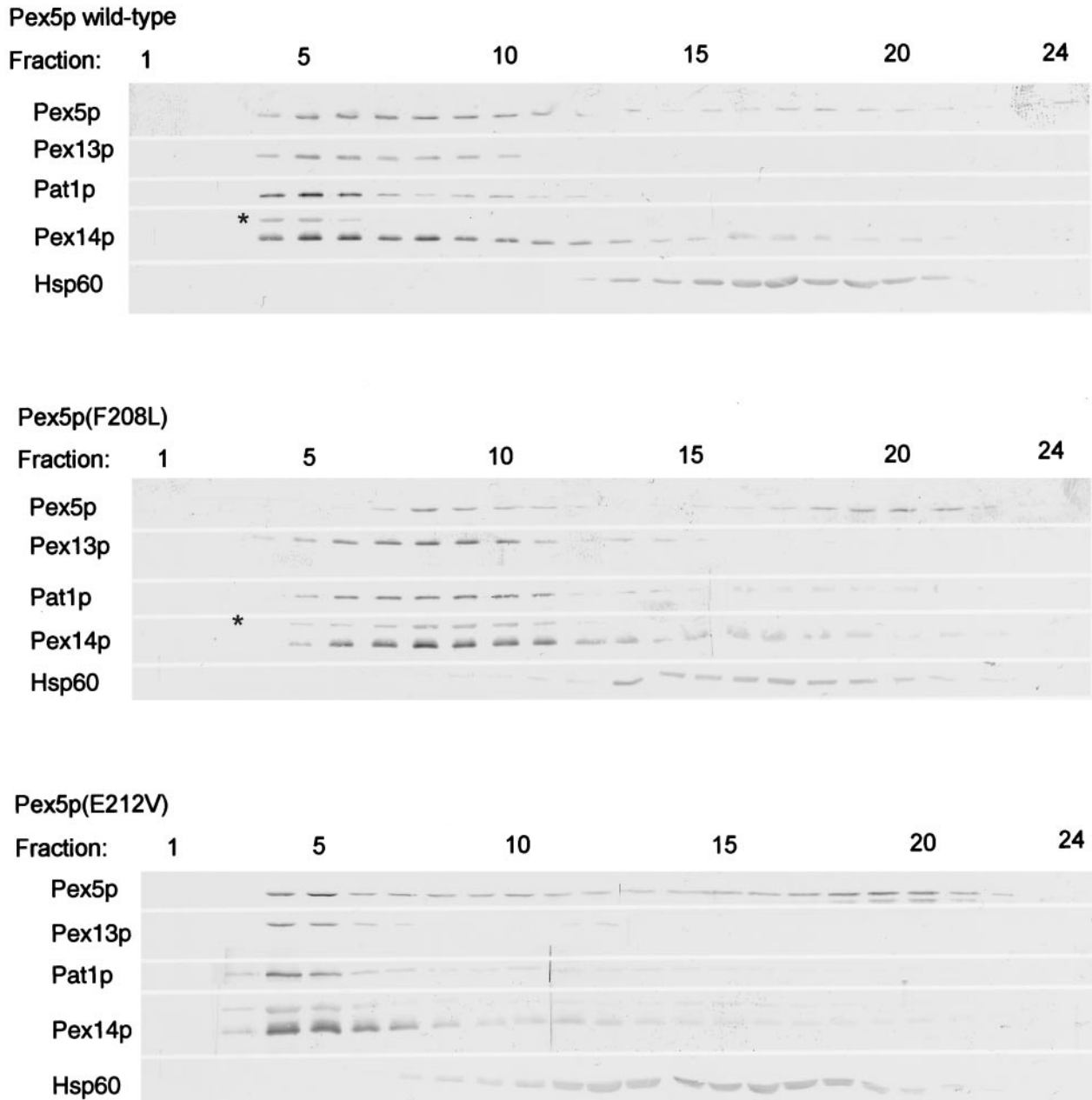
Figure 9. Pex5p mutants are associated with peroxisomes. 20,000 \times g pellet fractions of pex5 \Delta cells expressing wild-type Pex5p, Pex5p(F208L), or Pex5p(E212V) were loaded on top of a continuous Nycodenz gradient and centrifuged at 29,000 \times g in a vertical rotor for 2.5 h. Fractions of 0.5 ml were collected and analyzed by SDS-PAGE and Western blotting with antibodies specific for Pex5p; the peroxisomal membrane markers Pex13p, Pex14p, and Pat1p; and the mitochondrial marker Hsp60. Fraction 1 is the bottom of the gradient. The asterisk indicates a cross-reacting band.
