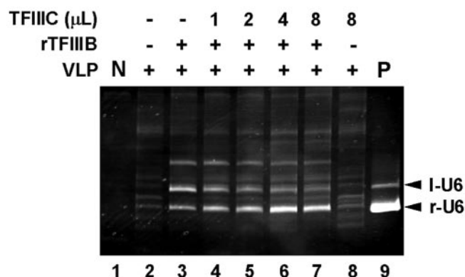
FIG. 4. TFIIC affects Ty3 integration by directing the assembly of TFIIB on the U6 promoter. Integration reactions were performed with 0.7–1.5 nM rTFIIIB subunits and 0.5–4.0 nM TFIIC (shown as multiples of 0.5 nM). PCR analysis of the integration products was performed as described in the legend to Fig. 2. Reactants are indicated at the top of the panel. Negative (N) and positive (P) controls are as described in the legend to Fig. 3.
