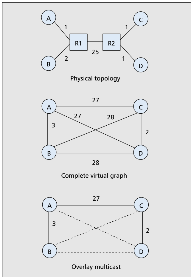
■ Figure 1. The physical and overlay topologies.
