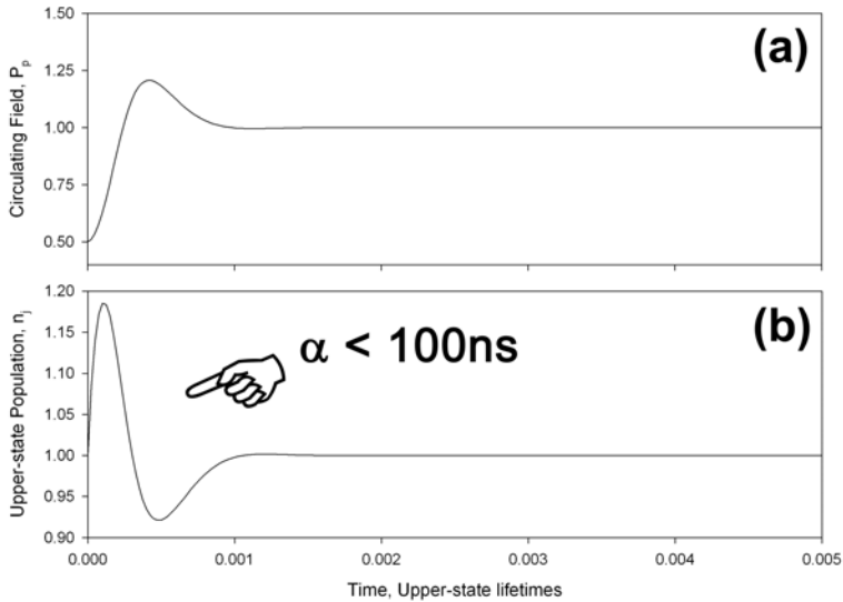
Fig. 22. Modelled transient response of an ICOPO operated internal to a VECSEL. Note that in order to ease comparison with previous figures, the time scale is in units of Nd:YVO 4 upper-state lifetime (100 \mu s).
