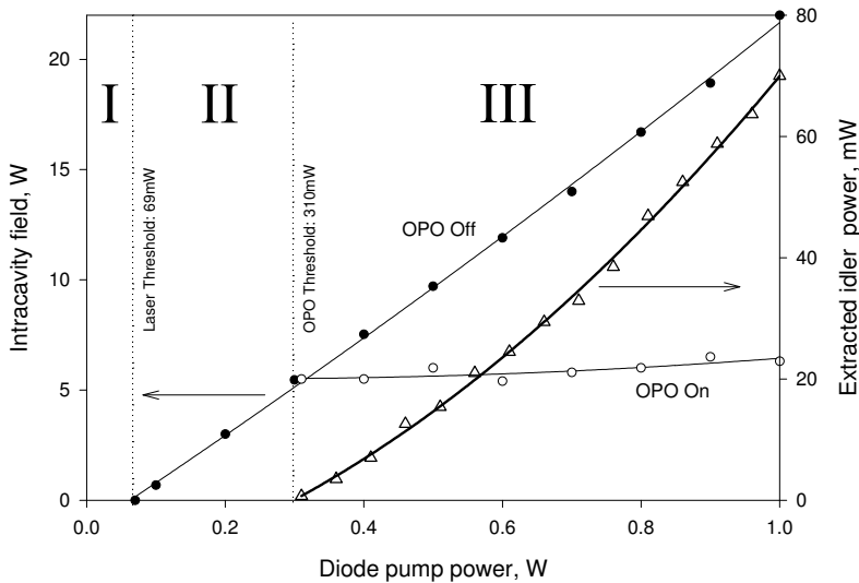
Fig. 10. Extracted idler (triangles) and pump-field with (open circles) and without (closed circles) operation of the OPO as primary diode pump power is varied. The idler wavelength was 3.66µm.
