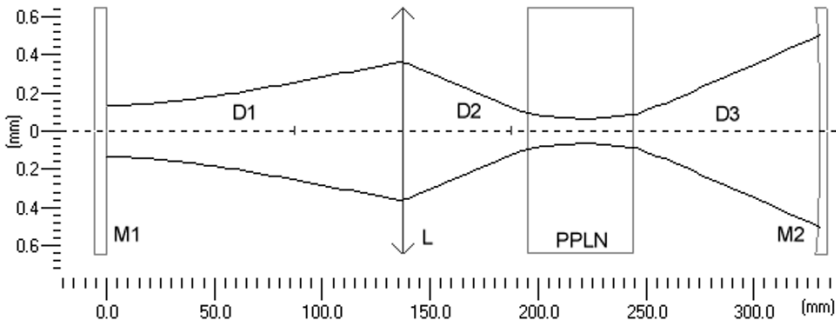
Fig. 7. Stability simulation of the pump cavity. Note that the beamsplitter has no focal power and is therefore omitted. Its optical length is incorporated into distance D2.
