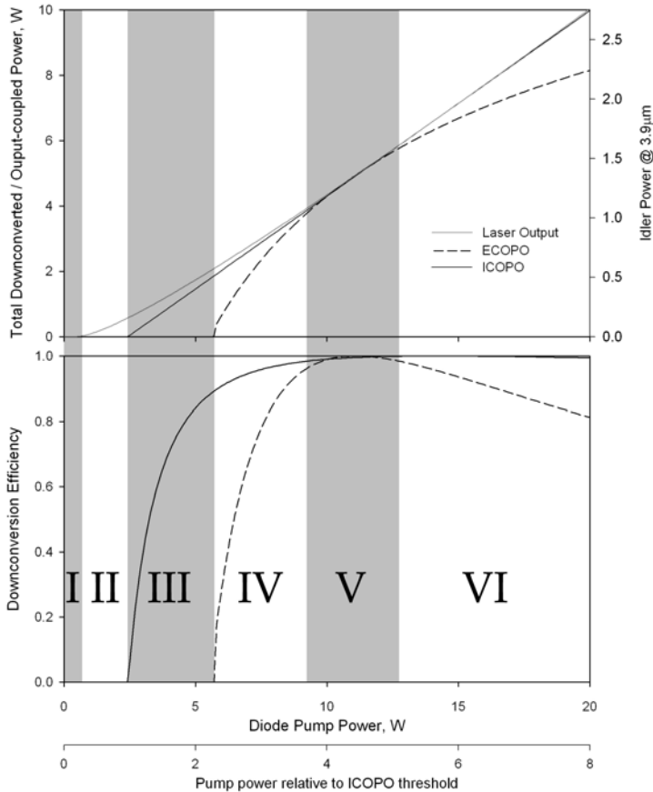
Fig. 4. Down-conversion characteristics of IC- and EC-OPOs
