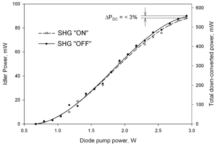
Fig. 21. SHG impact on down-converted power.
