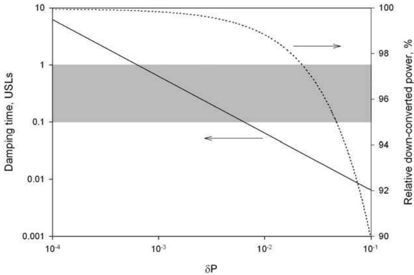
Fig. 18. The impact of increased \delta P upon damping time and down-converted power. The shaded region corresponds to the zone in which one would prefer to operate.
