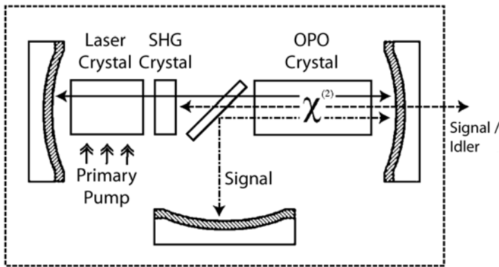
Fig. 16. CW ICOPO with SHG relaxation-oscillation suppression.
