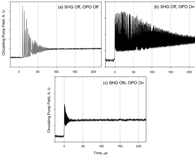
Fig. 20. Transient dynamics of (a) the laser alone, (b) the ICOPO without SHG and (c) the ICOPO with SHG.
