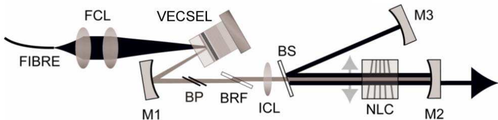
Fig. 23. VECSEL-based cw-ICOPO (Stothard, Hopkins et al. 2009).
