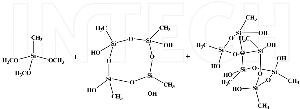
Figure 7. Introduction of POSS moiety by sol-gel method
