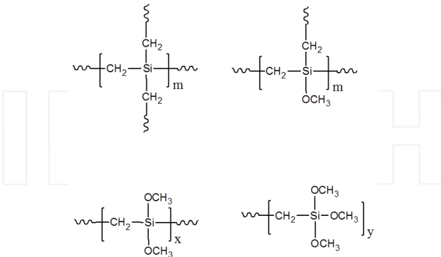
Figure 6. Chemical repeat units found in HBPCS precursors.
