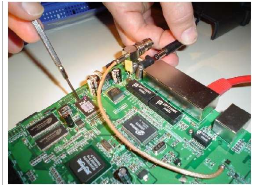
Figure 4: Unbricking the WRT54G (O'Donnell, 2004).
