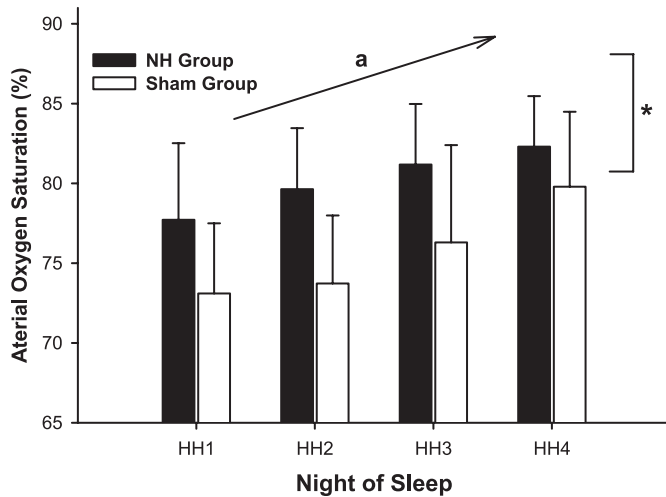
Fig. 4. SaO_2 during sleep under HH conditions. During sleep for the entire 4 nights under HH conditions, mean SaO_2 was higher for the NH group than for the sham group ( 80 \pm 4 vs. 76 \pm 4\% , *P < 0.05 ). For both groups, SaO_2 progressively increased from night 1 to night 4 (from 76 \pm 5\% to 81 \pm 4\% , ^aP < 0.05 ).
