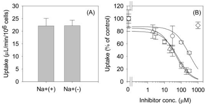
FIG. 4. Effect of \text{Na}^+ ion (A) and various compounds (B) on the uptake of telmisartan in isolated rat hepatocytes in the presence of 1% HSA. The substrate concentration used was 0.1 \mu\text{M} . Saturable uptake of telmisartan by isolated rat hepatocytes was determined using eq. 3 and eq. 4. B, data are shown as the percentage of the saturable uptake of telmisartan in the absence of inhibitors. Squares, triangles, circles, and diamonds represent the uptake of telmisartan in the presence of pravastatin, digoxin, taurocholate, and tetraethylammonium, respectively. Solid lines represent the fitted curves obtained by nonlinear regression analysis. Each bar and point represents the mean \pm S.E. of three separate determinations.
