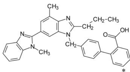
FIG. 1. Chemical structure of [ 3 H]telmisartan. The asterisk denotes the position of the 3 H-label.
