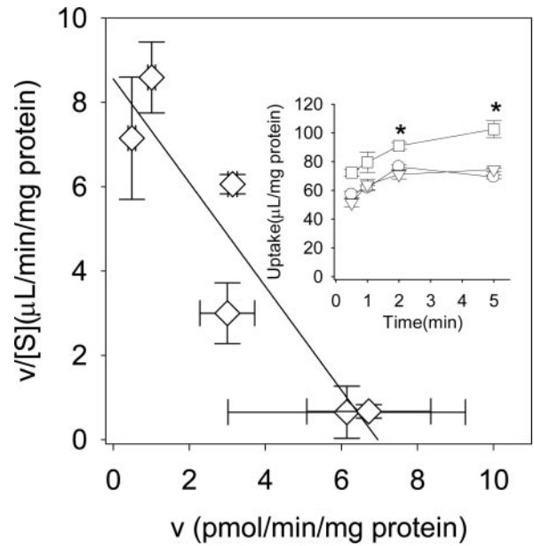
FIG. 6. Time profile and Eadie-Hofstee plot of the uptake of telmisartan into transporter-expressing cells in the absence of HSA. Inset, the substrate concentration used was 0.1 \mu\text{M} . Squares, triangles, and circles represent the uptake by OATP1B3-, OATP1B1-, and vector-transfected cells. The uptake of telmisartan by transporter-expressing cells was measured at a concentration between 0.05 and 10 \mu\text{M} telmisartan in the absence of HSA. The OATP1B3-mediated telmisartan transport was obtained by subtracting the uptake in vector-transfected cells from that in OATP1B3-expressing cells for 5 min. *, a significant difference ( P < 0.05 ) from the uptake by vector-transfected cells. Each point represents the mean \pm S.E. of three separate determinations.
