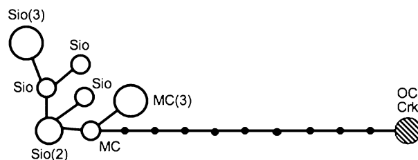
FIG. 5.—Haplotype network for haplogroup C-M130. Circle size reflects the frequency of that haplotype in this sample. White circles represent northeastern haplotypes, striped circles represent southeastern haplotypes, and small black circles represent intermediate haplotypes not identified in these samples. MC, Minnesota Chippewa; Sio, Sisseton/Wahpeton Sioux; OC, Oklahoma Red Cross Cherokee; Crk, Creek; Sem, Seminole.
