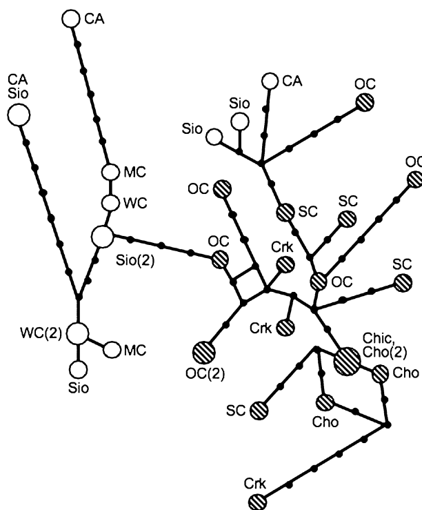
FIG. 4.—Haplotype network for haplogroup Q-M242*. Circle size reflects the frequency of that haplotype in this sample. White circles represent northeastern haplotypes, striped circles represent southeastern haplotypes, and small black circles represent intermediate haplotypes not identified in these samples. MC, Minnesota Chippewa; WC, Wisconsin Chippewa; Sio, Sisseton/Wahpeton Sioux; CA, Cheyenne/Arapaho; OC, Oklahoma Red Cross Cherokee; SC, Stillwell Cherokee; Chic, Chickasaw; Cho, Choctaw; Crk, Creek.
