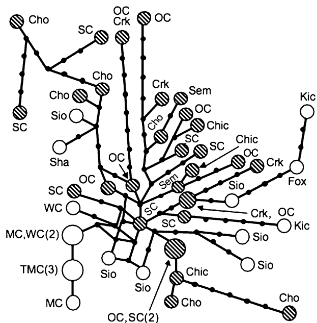
FIG. 3.—Haplotype network for haplogroup Q-M3*. Circle size reflects the frequency of that haplotype in this sample. White circles represent northeastern haplotypes, striped circles represent southeastern haplotypes, and small black circles represent intermediate haplotypes not identified in these samples. MC, Minnesota Chippewa; WC, Wisconsin Chippewa; Sio, Sisseton/Wahpeton Sioux; OC, Oklahoma Red Cross Cherokee; SC, Stillwell Cherokee; Chic, Chickasaw; Cho, Choctaw; Crk, Creek.
