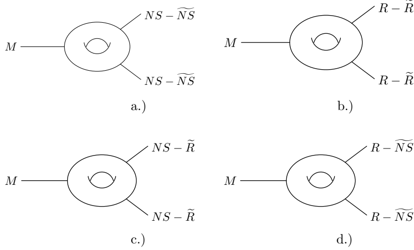
Figure 4: The 4 possible contributions to \mathcal{A}_{M^{**}}^{\text{tree}} .
