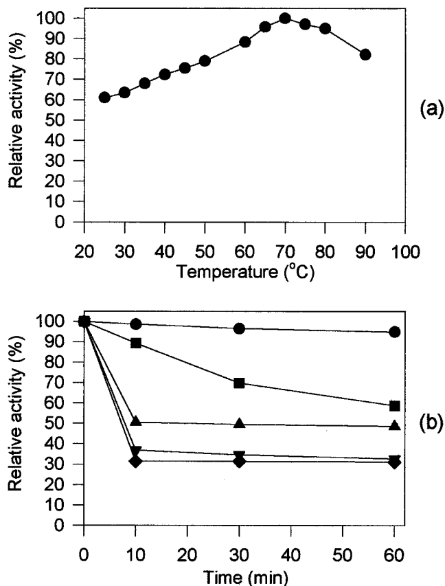
FIG. 2. Effect of temperature on fibrinolytic activity (a) and stability (b) of CK at pH 10.0. (b) ●, 40°C; ■, 50°C; ▲, 60°C; ▼, 70°C; ◆, 80°C.
