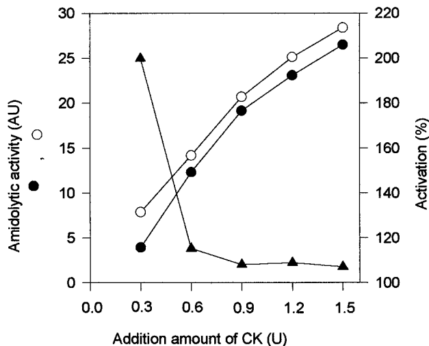
FIG. 5. Amidolytic activity of CK and a mixture of CK and plasminogen with chromogenic substrate (H-D-Val-Leu-Lys-pNA). ●, CK; ○, CK and plasminogen (0.5 U).
