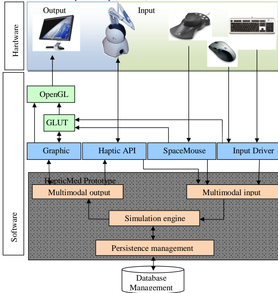
Figure 1. HUI the interconnections among the software components and the hardware components involved
