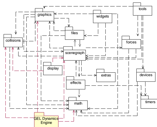
Figure 5. CHAI3D framework – architecture
