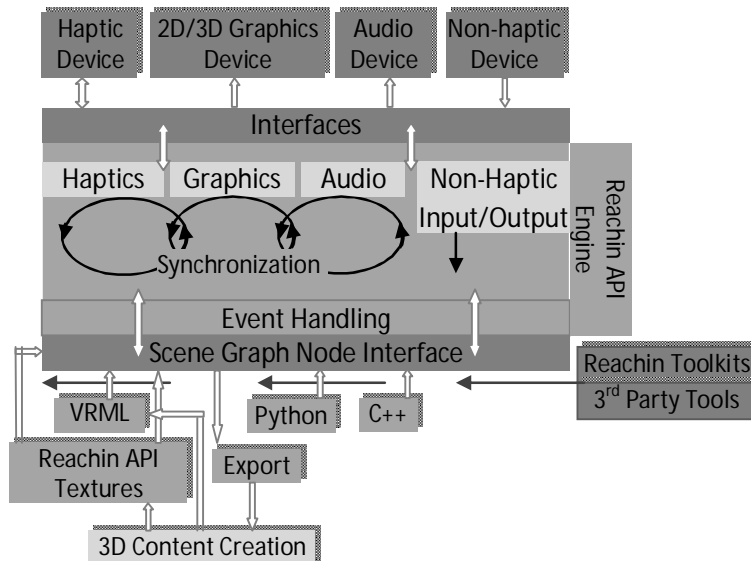
Figure 3. ReachIn API – architecture
