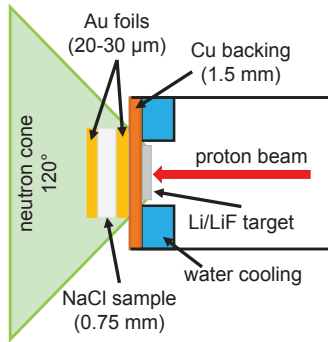
FIG. 1. Schematic of the activation set-up at KIT.
