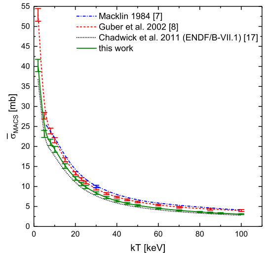
FIG. 5. MACS from this work for energies between kT = (2-100) \text{ keV} compared to the values of Macklin [7] and Guber et al. [8], and the results obtained directly with the resonance parameters from ENDF/B-VII.1 [17].
