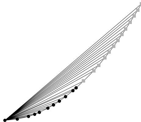
Fig. 2. Points on a parabola.
