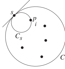
Fig. 1. The points s and p_i are Delaunay neighbors.
