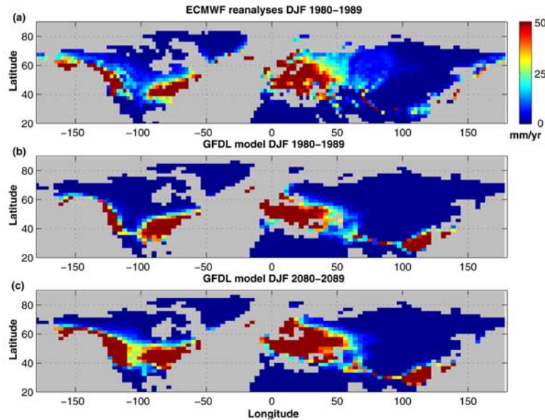
Figure 2. (a) Average wintertime ROS amounts for 1980–1989, calculated using daily reanalysis data from the European Centre for Medium Range Forecasting (ECMWF) [Gibson et al. , 1996]. Only data from December, January and February are used. To make the plots clearer, the color scale maximizes at 50 mm/yr. (b), as for panel (a), but using the output from the GFDL global climate model. (c), as for panel (b) but for GFDL climate model predictions for 2080–2089 under a standard anthropogenic climate forcing scenario of a 1% per year increase in \text{CO}_2 . For the GFDL model monthly-mean model output was used as daily output was not available. ROS was calculated from the model output fields of snow depth, snowfall, and total precipitation. Note that the model grid size in the GFDL and ECMWF output are slightly different.
