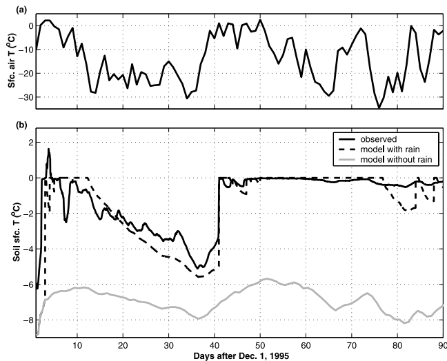
Figure 1. (a) Air temperature measured at 1.6 m above the soil surface. (b) Observations (solid line) and modeling (dashed and gray lines) of soil surface temperatures [Putkonen, 1998] at our field site near Ny-Ålesund, Spitsbergen, winter 1995–1996. The sharp upward spikes in the observed record (solid dark line) show the impact and timing of the two major rain events during this period. The gray line is integration of a permafrost evolution model that does not include the impact of rain events. The dashed line is the integration of the permafrost model including rain events [Putkonen, 1998]. Using meteorological data from the nearby (10 km) Ny Ålesund station, and summing the totals of the reported rain events and half the totals of reported mixed rain/snow events, around 180 mm of rainfall was reported over the winter. Because of local-scale variations the input of liquid water at the site is not always certain. In this figure the magnitude (but not timing) of rain added to the model was varied to optimize the match to the observations. The integration shown (dashed line) used a total of 173 mm, which therefore compares favorably to the observations. The snow and soil thermal parameters in the model were held fixed. Snow depth ranged between 0.3 and 1.7 m (mean 1.3 m) during the period.
