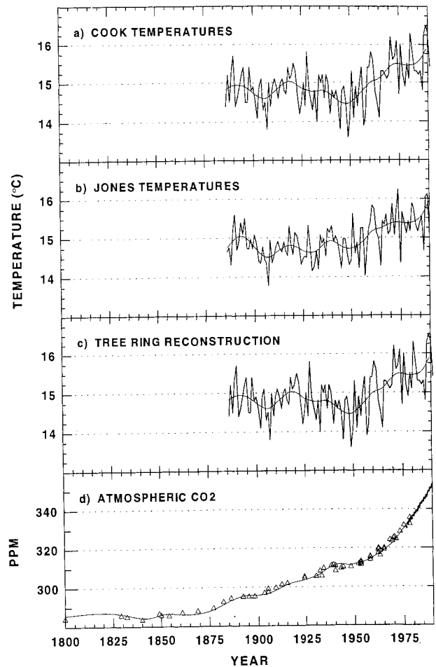
FIG. 2 — A comparison of the reconstructed temperatures (C) with two independently derived warm-season instrumental temperature records (A, B) for Tasmania. The common period is 1886–1989. The yearly values have superimposed upon them smoothed curves that highlight longer-term trends in the records. Also shown are atmospheric \text{CO}_2 trends derived from Law Dome ice cores ( \Delta ), Cape Grim monthly averages ( \bullet ) and a smoothing spline with 50% attenuation at 50 years (line). Note — the Cape Grim data are normalised to the 1957–90 South Pole data of Keeling et al. (1989) which, on this scale, are indistinguishable from the spline fit.
