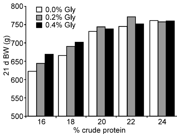
Fig. 1: Influence of dietary crude protein level and supplemental Gly on 21 d body weight of male broilers fed diets calculated to provide recommended levels of essential amino acids (NRC, 1994)
