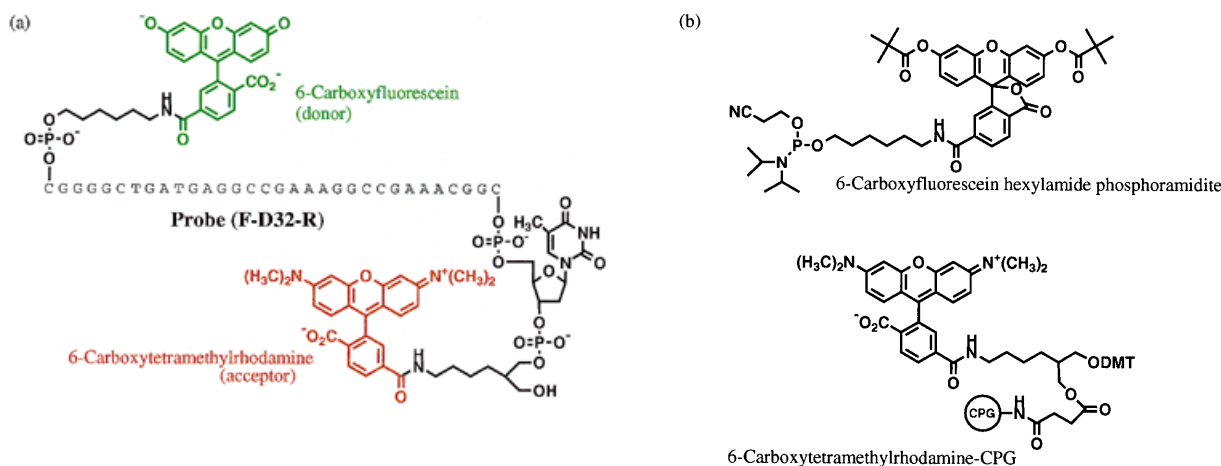
Figure 3. Structures of the probe (a) and reagents (b) for the synthesis of the probe (F-D32-R). The 32mer deoxyribonucleotide probe F-D32-R was modified with two fluorophores, namely 5'-6-carboxyfluorescein and 3'-6-carboxytetramethylrhodamine.
