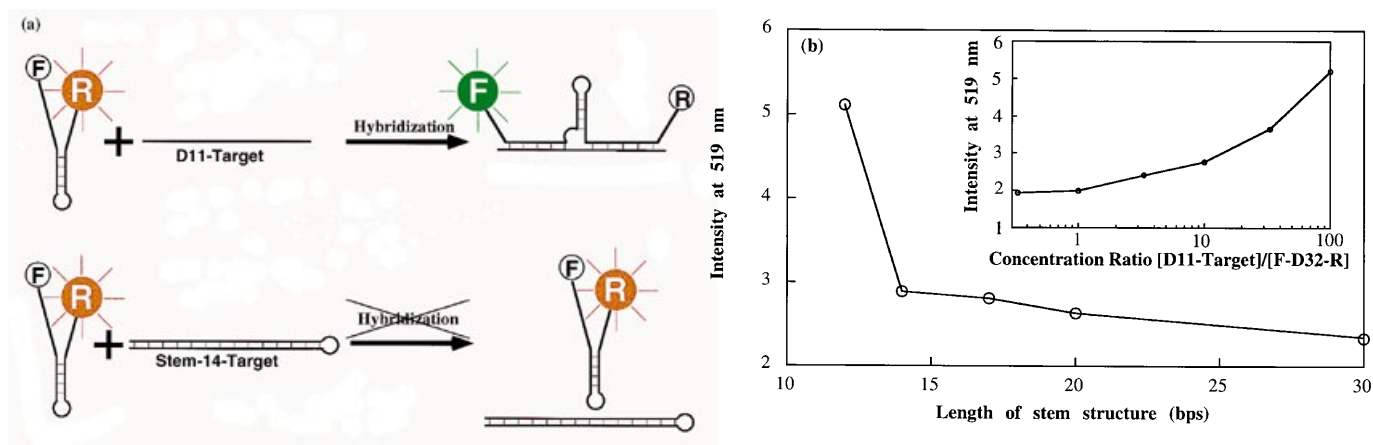
Figure 9. (a) Interaction of the hammerhead-ribozyme-shaped F-D32-R either with a linear target that mimicked a ribozyme substrate (D11-Target) or with a highly structured substrate (Stem-14-Target). When F-D32-R is mixed with D11-Target, FRET is expected to decrease as a result of hybridization. By contrast, the incubation with a stable stem-Target is not expected to lead to a decrease in FRET because of failure of hybridization. (b) Effects of the length of the duplex structure within the Stem-Target on the decrease in FRET. After a 70 min incubation of 30 pmol of F-D32-R with 3 nmol of stem-Target with various lengths, the intensity at 519 nm was measured. It was apparent that F-D32-R had hybridized to Stem-12-Target, but not to Stem-Targets with >14 bp in the stem. The inset shows the dose dependence of increase in the intensity at 519 nm after a 70 min incubation of 30 pmol of F-D32-R with D11-Target.
