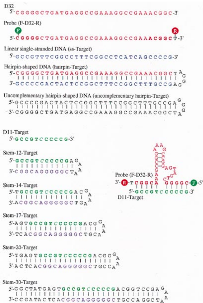
Figure 4. Sequences of the probe and the target molecules. The sequence of the probe corresponded to that of the 32mer hammerhead ribozyme (37–40). Nine target DNAs were used in this study. Linear single-stranded DNA (ss-Target), hairpin-shaped DNA (hairpin-Target), and hairpin-shaped DNA without complementary sequence (uncomplementary hairpin-Target) were used for investigations of the interactions between the non-structured probe and non-structured or structured targets. D11-Target and Stem-##-Targets were used for studies of hybridization between the structured probe and non-structured or structured targets. Bold letters indicate sites of hybridization with the probe. The secondary structure of the probe that hybridized to D11-Target is shown in the middle of the Figure on the right.
