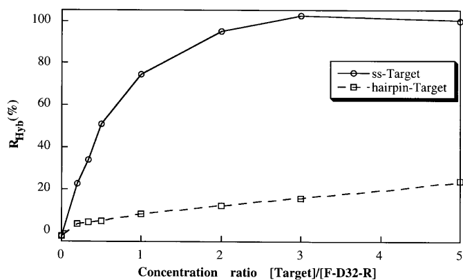
Figure 8. Dose-dependent changes in R_{Hyb} . Various amounts (0, 6, 10, 15, 30, 60, 90 and 150 pmol) of ss-Target (solid line) or hairpin-Target (broken line) were incubated with 30 pmol of F-D32-R for 70 min. The amount of the target strand apparently affected the extent of R_{Hyb} in a dose-dependent manner.
