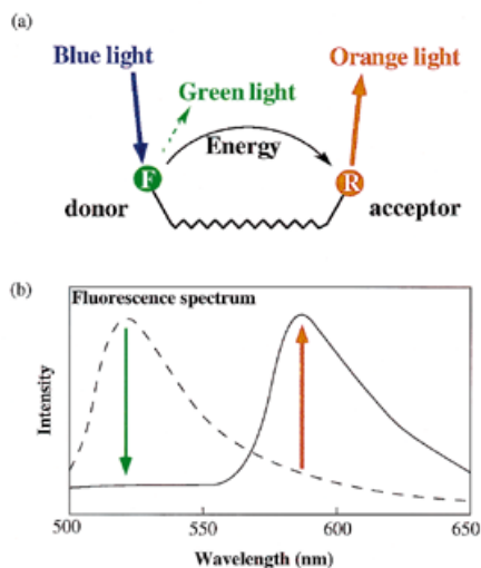
Figure 1. Fluorescence resonance energy transfer. (a) When the fluorescence spectrum of one fluorophore (donor; F) overlaps with the excitation spectrum of the other fluorophore (acceptor; R), the excitation of the donor induces the emission of fluorescence from the acceptor, while its own fluorescence decreases. (b) In this study, 6-carboxyfluorescein and 6-carboxytetramethylrhodamine were employed as the donor and the acceptor, respectively. When fluorescence resonance energy transfer (FRET) takes place, the excitation of 6-carboxyfluorescein by blue light (492 nm) results in the emission of orange light (586.5 nm) from 6-carboxytetramethylrhodamine, while the emission of green light (519 nm) from 6-carboxyfluorescein decreases.
