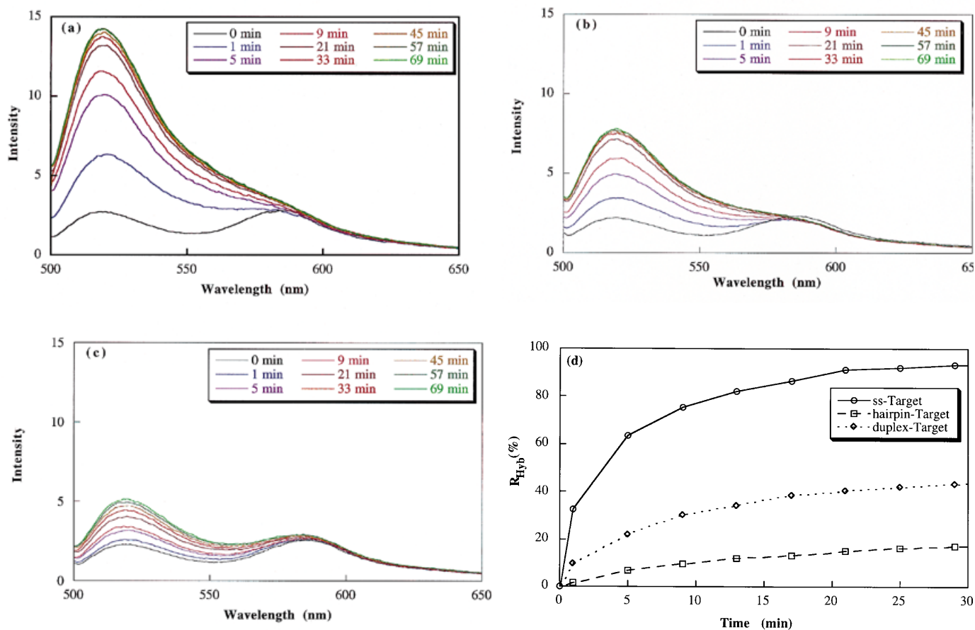
Figure 7. Time-dependence of changes in FRET. (a), (b), (c) Typical time-courses of changes in the fluorescence spectra of a 1 ml solution of probe (30 nM) after the addition of 150 pmol of ss-Target, of duplex-Target generated by mixing 150 pmol of ss-Target and the same amount of D32, and of 150 pmol of hairpin-Target, respectively. (d) The increase in the peak emission intensity (as a percentage) at 519 nm (denoted as R_{Hyb} ) was employed as the measure of the extent of hybridization. Time-courses are shown for changes in R_{Hyb} at 30 min after the addition of either ss-Target (solid line), duplex-Target (dashed line) or hairpin-Target (broken line).
