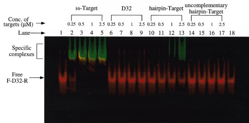
Figure 6. Typical gel image of gel-shift assays analyzed by a fluorescence imaging analyzer. In the solution containing 10 mM Tris-HCl (pH 7.4), 0.1 M NaCl, 5 mM MgCl 2 , and 10 mM EDTA, 400 nM of the probe and none (lanes 1 and 18), 250 nM (lanes 2, 6, 10 and 14), 500 nM (lanes 3, 7, 11 and 15), 1000 nM (lanes 4, 8, 12 and 16) and 2500 nM (lanes 5, 9, 13 and 17) of each target were incubated for 70 min and followed by a 12% native PAGE. Resultant gels were analyzed by a fluorescence imaging analyzer and the level of fluorescence at 530 nm and that at 590 nm were calculated by a computer program (FluorSep, Molecular Dynamics, CA). The green and red bands indicate the fluorescence at 530 and 590 nm, respectively. The decrease in the extent of FRET (red color) is accompanied by the increase in the shifted band (green color).
