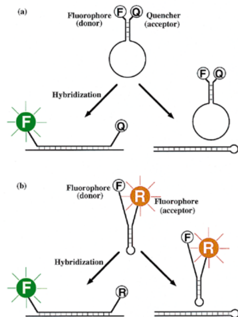
Figure 2. Detection of hybridization by the use of molecular beacons and by our probes. (a) Labeled oligonucleotides with a fluorophore as a donor (F) and a quencher (Q) as an acceptor can be used to identify the presence of a complementary sequence in solution (27). Successful hybridization of the molecular beacon with the target results in emission from the donor. (b) Monitoring of the integrity of oligonucleotides in vitro and in vivo is possible by exploiting the FRET between two different fluorochromes attached to a single oligonucleotide (22), which can also be used to detect hybridization. Our probe used in this study (Fig. 1a) in a single-stranded form is detectable as a result of emission from the acceptor (R) that could be excited directly by an appropriate light source or by transfer of energy from the donor. In the case of molecular beacons, probes are dark when free in solution but they fluoresce brightly when hybridized to targets. In the case of our probes, the extent of FRET is maximal when probes are free in solution and a decrease in FRET indicates successful hybridization.
