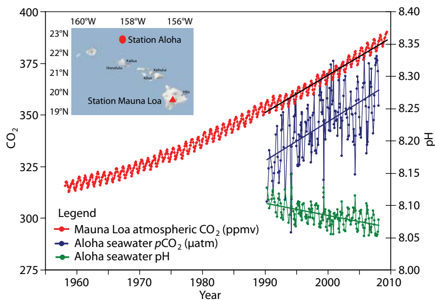
Figure 1: Time series of atmospheric CO 2 at Mauna Loa (in parts per million volume, ppmv; red), surface ocean pCO 2 (μatm; blue) and surface ocean pH (green) at Ocean Station ALOHA in the subtropical North Pacific Ocean. Note that the increase in oceanic CO 2 over the past 17 years is consistent with the atmospheric increase within the statistical limits of the measurements. Mauna Loa data courtesy of Pieter Tans, National Oceanic and Atmospheric Administration/Earth System Research Laboratory ( http://www.esrl.noaa.gov/gmd/ccgg/trends/ ); Hawaii Ocean Time-Series (HOT)/ALOHA data courtesy of David Karl, University of Hawaii ( http://hahana.soest.hawaii.edu/ ; see also Dore et al., 2009)
