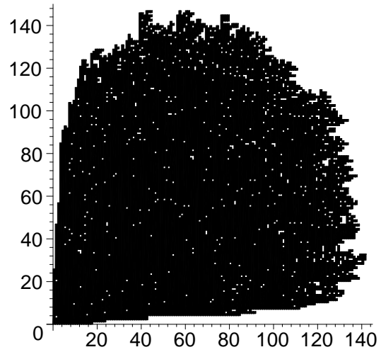
Figure 5.6: C(400) for d = 2 and the Pareto distribution F(x) = \min(0, 1 - x^{-3/4}) , which has infinite mean.
