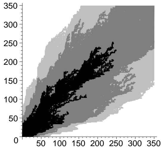
Figure 5.4: C(t) , t = 18, 36, 54 , with d = 2 and X = 0 w.p. 0.645 and X = (0.355)^{-1} w.p. 0.355 (showing only the intersection with the box [0, 350]^2 ). Here h(\mathbf{x}) = 0 for some (though not all) \mathbf{x} ; thus the asymptotic shape is non-compact (but not the whole of \mathbb{R}_+^d ), and a.s. the set C(t) will be infinite for some t .
