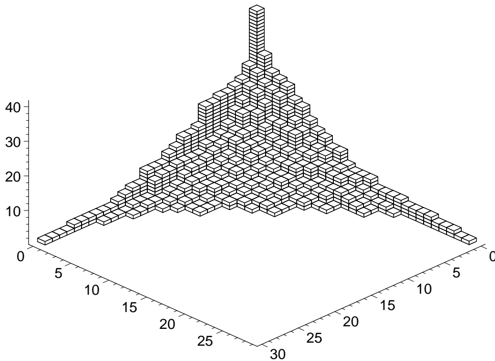
Figure 5.7: B(30) for d = 3 and F exponential with mean 1.
