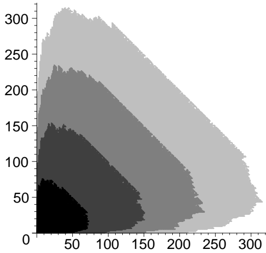
Figure 5.5: C(t) , t = 50, 100, 150, 200 , with d = 2 and X = 0.5 w.p. 0.8, X = 3 w.p. 0.2.
