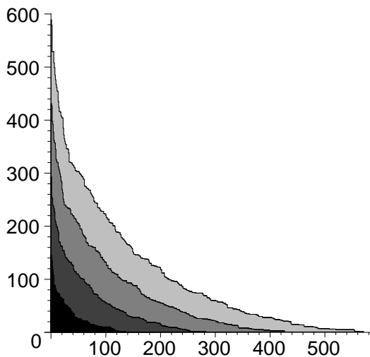
Figure 5.1: Simulation of the last-passage process B(t) , t = 150, 300, 450, 600 , for d = 2 and F exponential with mean 1. Here the asymptotic shape B is known to be \{(x, y) \in \mathbb{R}_+^2 : \sqrt{x} + \sqrt{y} \leq 1\} .
