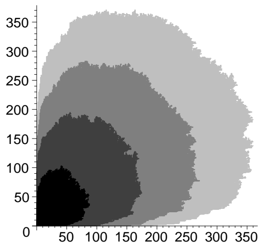
Figure 5.2: First-passage process C(t) , t = 50, 100, 150, 200 for d = 2 and F exponential with mean 1.
