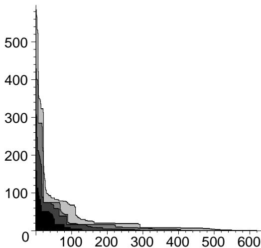
Figure 5.3: B(t) , t = 150, 300, 450, 600 , with d = 2 and the Pareto distribution F(x) = \min(0, 1 - (3x)^{-3/2}) , which has mean 1 but infinite variance. The asymptotic shape B consists only of two lines, between the origin and (0,1) and between the origin and (1,0) .
