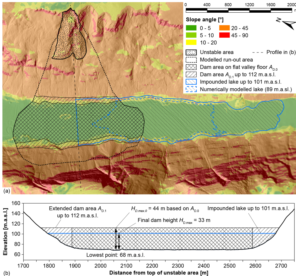
Figure 9. Iterative procedure to estimate the maximum dam height H_{D,max} using the modelled run-out area to estimate the dam area A_D . The example shown is the 21 \times 10^6 \text{ m}^3 rockslide of Gamanjuni 3 in northern Norway (Böhme et al., 2016), which might lead to a 33 m high landslide dam using Eq. (4) with the iterative procedure to assess the possible dam area A_D .
