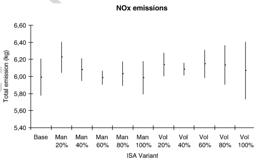
Fig. 7. Emissions of NO x of the total network. Symbols are as in Fig. 6.
