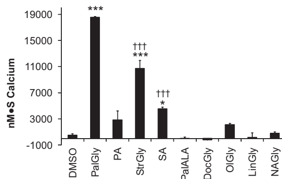
Fig. 4. PalGly induced calcium influx in F-11 cells with strict structural requirements. Comparison of PalGly-induced calcium influx with calcium influx by structurally related molecules. Calcium influx was calculated from the integral of the time \times calcium-concentration curve as described in the text. Free glycine was tested at 16 \mu\text{M} . All other compounds were tested at 10 \mu\text{M} . One-way ANOVA with Bonferroni's post hoc test. *, p < 0.05 compared with vehicle; ***, p < 0.001 compared with vehicle; †††, p < 0.001 compared with PalGly.
