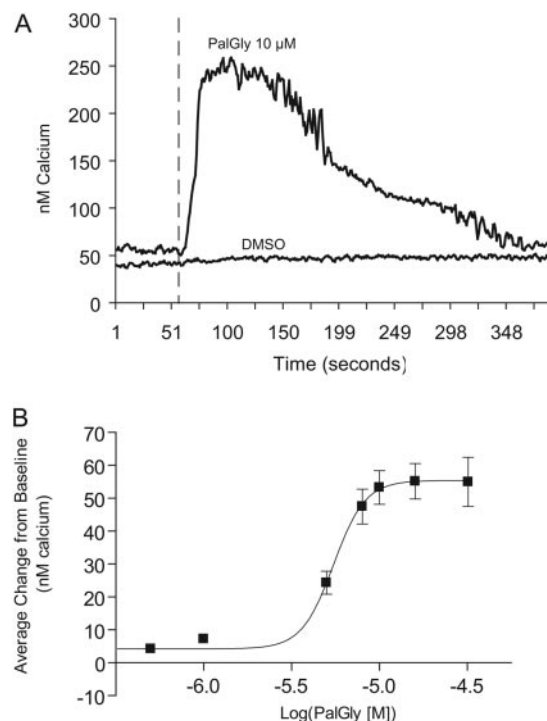
Fig. 3. PalGly induced a dose-dependent calcium influx in F-11 cells. A, single cell calcium traces (assessed by Fura-2 fluorescence) of F-11 cells treated with either 10 \mu\text{M} PalGly or DMSO. Dashed line indicates the time of drug administration. B, a dose-response curve of F-11 cells to PalGly. The following formula was used to calculate the average change in nanomolar calcium for each cell: [(the average response 60 s after PalGly application) – (the average response 60 s before PalGly application)]. All cells, regardless of their response rate, were averaged. Each data point represents an average of single cells ( n = 31\text{--}75 ) from at least three independent plates. The \text{EC}_{50} value for PalGly = 5.5 \mu\text{M} . Error bars indicate S.E.M.
