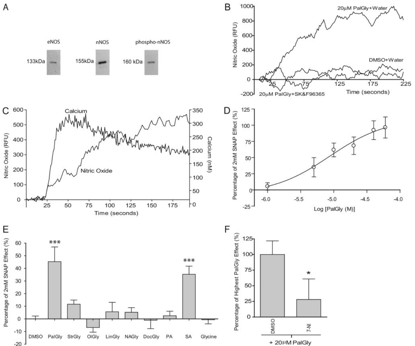
Fig. 7. PalGly treatment induced NO production in F-11 cells in a calcium-dependent manner. A, F-11 cells express calcium-dependent NOS isoforms. Western blots showed that eNOS, nNOS, and Ser847-phospho-nNOS were present in F-11 cells. iNOS was not detected using Western blotting. B, NO release by F-11 cells upon PalGly treatment is calcium channel-dependent. Traces from individual wells containing DAF-2-loaded F-11 cells displayed an increase in NO upon treatment with PalGly but not DMSO. Treatment of F-11 cells with the nonspecific calcium channel blocker SK&F96365 (20 \mu M) suppressed PalGly-evoked NO release compared with vehicle (water)-treated cells. Data points are presented as the increase in fluorescence relative to baseline using a 9-point moving point average. C, NO production closely parallels calcium influx in F-11 cells. A calcium trace from a single cell is overlaid with a NO trace from a single well. D, PalGly causes dose-dependent release of NO in F-11 cells. Data are presented as a percentage of the effect of 2 mM SNAP in 5 \mu M DAF-2. PalGly at and above 10 \mu M caused significant elevations in NO release compared with DMSO (**, p < 0.01 , n = 6 , one-way ANOVA, Dunnett's t test, post hoc). The EC_{50} value for the effect of PalGly was 8.7 \mu M. E, NO release by PalGly in F-11 cells had rigid structural requirements. PalGly and stearic acid (SA), but not other structurally related compounds, significantly increased NO production compared with DMSO vehicle (***, p < 0.001 , n \geq 9 , one-way ANOVA, Dunnett's t test, post hoc). All compounds were tested at 10 \mu M. Data are presented as a percentage of the effect of 2 mM SNAP in 5 \mu M DAF-2. F, NOS catalyzes PalGly-induced NO production. PalGly-induced NO production in F-11 cells was inhibited by pretreatment of cells with 200 \mu M 7-NI, a NOS inhibitor (*, p < 0.05 , n = 32 , one-way ANOVA, LSD post hoc test). Data are presented as a percentage of the maximum mean effect of PalGly in each experiment, which occurred in each case under DMSO treatment conditions. Error bars represent S.E.M.
