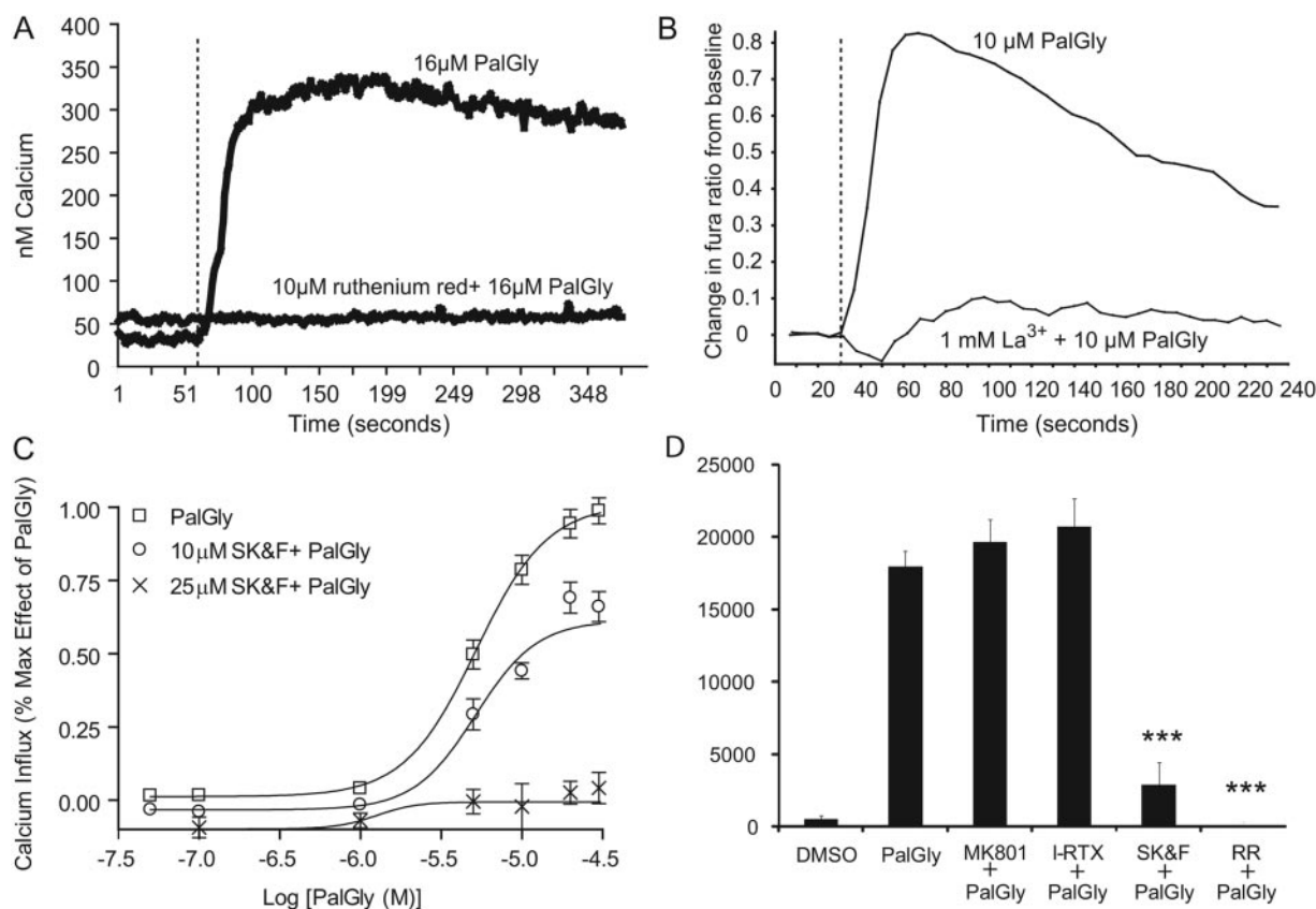
Fig. 6. PalGly-induced calcium influx was inhibited by pretreatment with ruthenium red (10 μM), SK&F96365 (25 μM), and La 3+ (1 mM). A, single cell calcium traces for F-11 cells treated with 16 μM PalGly after administration of vehicle or 10 μM ruthenium red. B, a representative F-11 well population calcium influx of cells pretreated with La 3+ or vehicle. C, concentration-response curves for PalGly and PalGly + SK&F96365 (10 or 25 μM) show profound inhibition of PalGly-induced calcium influx in F-11 cells after treatment with 25 μM SK&F96365. n = 3–20 wells per condition. D, PalGly (16 μM) induced marked calcium influx in the presence of MK801 (25 μM) and I-RTX (35 nM), whereas it lacked efficacy in the presence of SK&F96365 (10 and 24 μM) or ruthenium red (10 μM). Calcium mobilization was calculated from the integral of the calcium concentration \times time curve as described in the text. ***, p < 0.001 difference from vehicle + PalGly. One-way ANOVA with LSD post hoc tests. Error bars indicate S.E.M.
