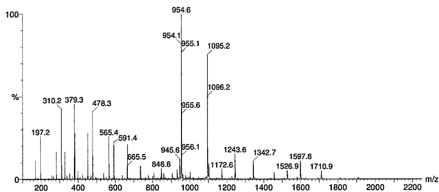
FIG. 3. ESI tandem MS of the [M + 2H]^{2+} molecular ion at m/z 1,095.2.
