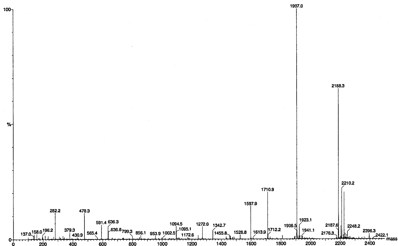
FIG. 2. MS analyses of SP508A using single-stage ESI MS (upper panel) and with MaxEnt3 deconvolution (lower panel).
