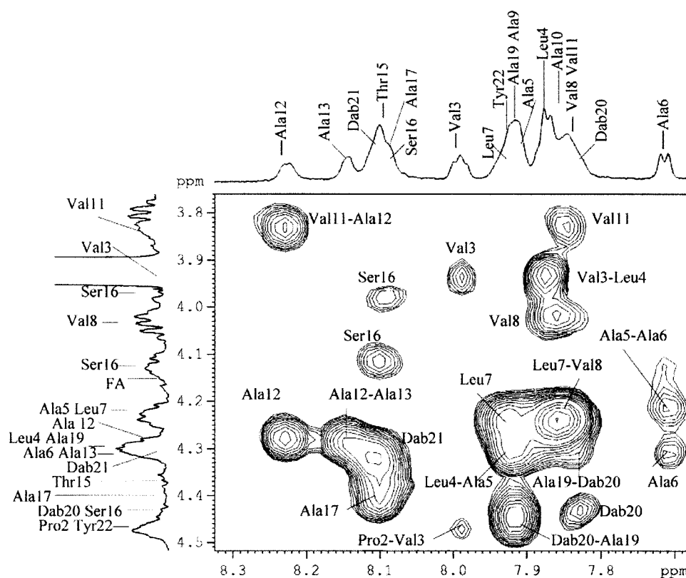
FIG. 4. Slice of ^1\text{H} - ^1\text{H} NOESY map of SP508A in TFE/ \text{H}_2\text{O} (4:1, vol/vol) at 300 K. The major connections leading to the amino acid sequence are highlighted. In the F1 and F2 dimensions, the ^1\text{H} NMR spectrum in TFE/ \text{H}_2\text{O} (4:1, vol/vol) at 300 K is reported.
