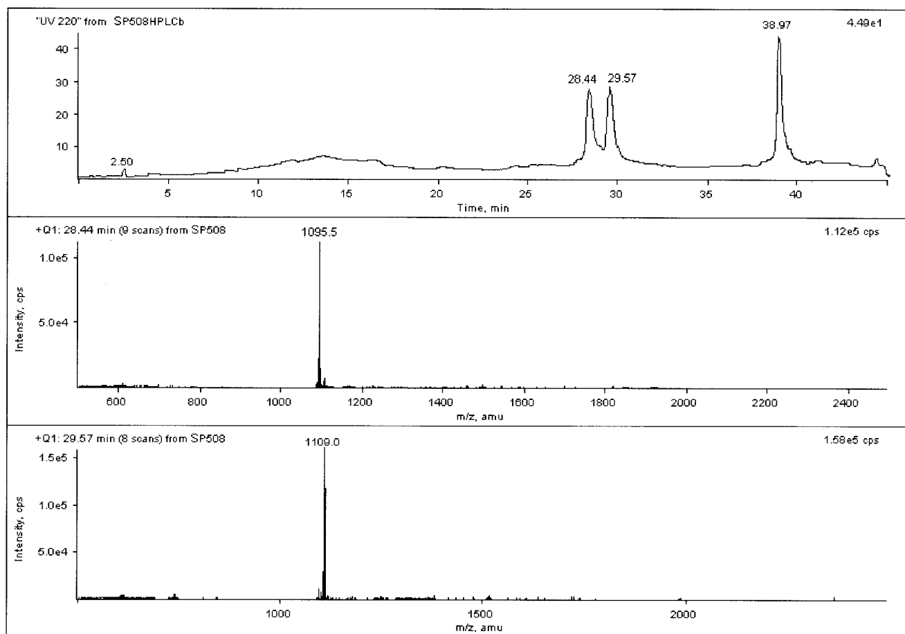
FIG. 1. Total ion current chromatogram of the prepurified culture of P. syringae pv. lachrymans strain 508 filtrates (upper panel) and mass spectra of SP508A (middle panel) and SP508B (lower panel). amu, atomic mass units.
