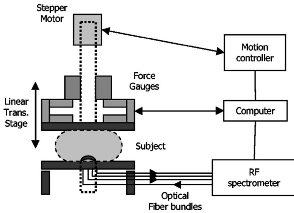
Fig. 1 Experimental setup. A computer-controlled translation stage applies compression to a subject's breasts while frequency domain optical measurements are acquired through one source and three detector fibers. Force transducers are integrated into the compression frame for monitoring.
