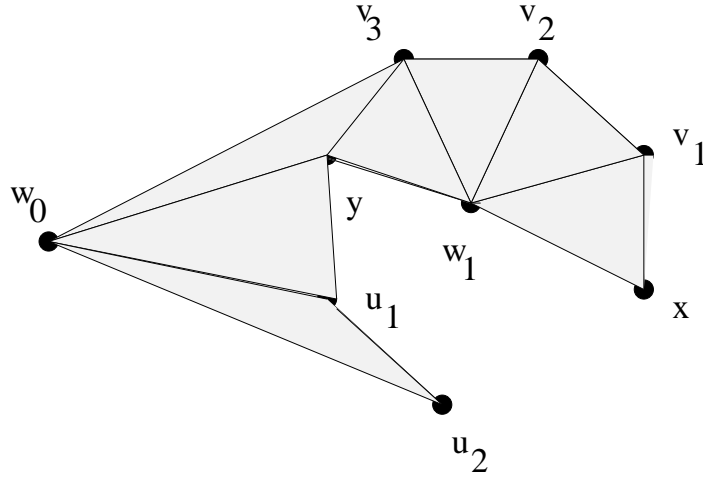
FIGURE 8. The tree S in the link of \rho'_0
