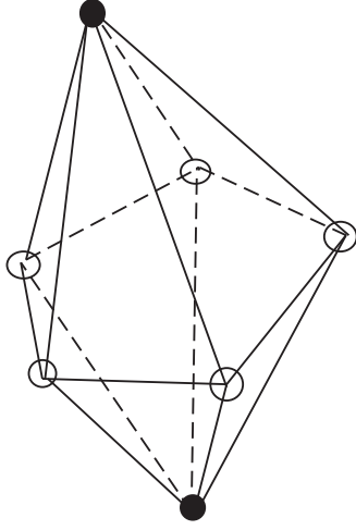
FIGURE 1. Balanced bipyramid, \phi(\bullet) = 1, \phi(\circ) = 2 .
