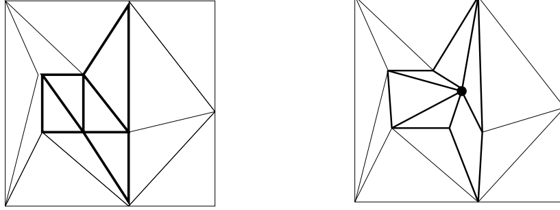
FIGURE 5. Central retriangulation of a simple 2-tree
