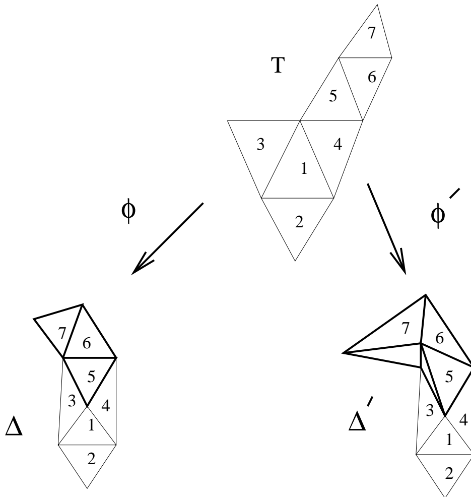
FIGURE 7. Creating a spanning simple (d - 1) -tree
