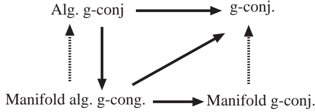
FIGURE 4. Various g -conjectures
