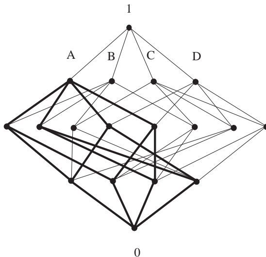
FIGURE 3. Hasse diagram of P .
