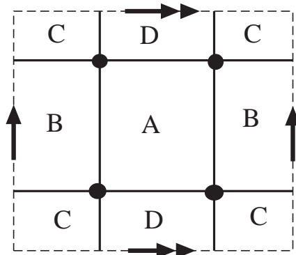
FIGURE 2. Cell decomposition of the torus
