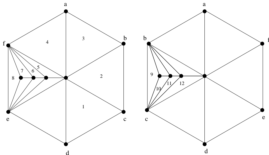
FIGURE 6. Spanning 2-tree in the link of an edge of \Delta_{K3}
