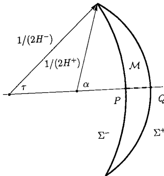
Figure 1: Moon domain; H^- \neq H^+ .
