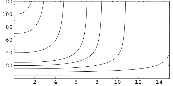
Fig. 2. Plot of the Lorentz factor \Gamma = (1 - \dot{X}^2 - kX^2/2)^{-1/2} versus T/(GM) based on integration of equation (14) with initial data X = 0 at T = 0 with \dot{X}(0) = (\Gamma_0^2 - 1)^{1/2}/\Gamma_0 corresponding respectively to \Gamma_0 = 5, 10, 15, 20, 25, 40, 70 and 100 . In this plot a/(GM) = 1 and r_0/(GM) = 15 . The graph illustrates acceleration of the particle such that \Gamma essentially approaches infinity at T/(GM) \approx 11, 9, 7, 5, 3 and 2.6 for \Gamma_0 = 15, 20, 25, 40, 70 and 100 , respectively.
