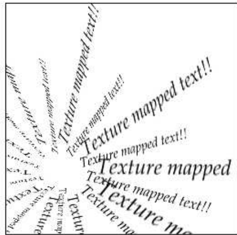
Figure 3. Anti-aliased text.
