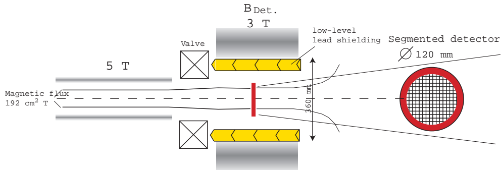
Figure 18: Schematic view of the detector area with magnet configuration and position of the electron detector.
