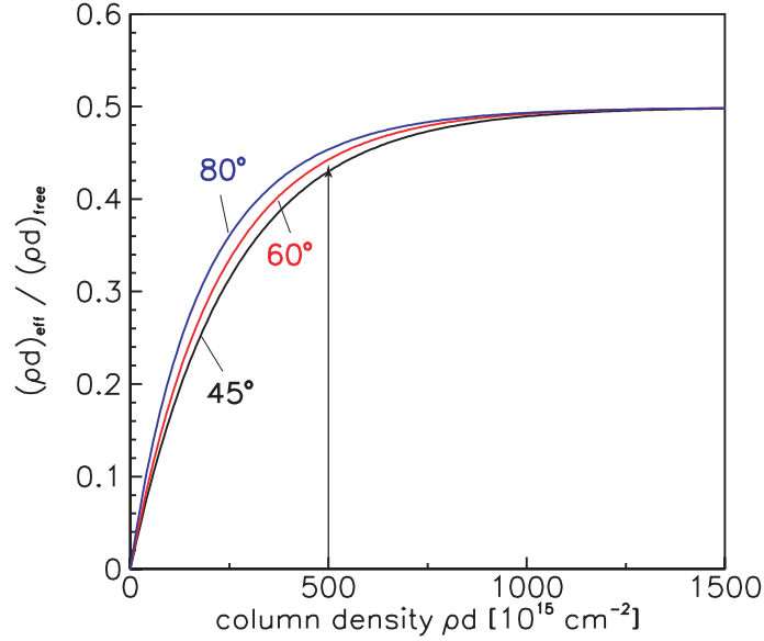
Figure 12: Ratio of effective to free column density (\rho d)_{\text{eff}}/(\rho d)_{\text{free}} (being proportional to the signal rate S ) as function of the source column density \rho d for different maximum accepted starting angles \theta_{\text{max}} . The vertical line indicates the proposed WGTS parameters of \rho d = 5 \cdot 10^{17} molecules/cm 2 and \theta_{\text{max}} = 51^\circ .
