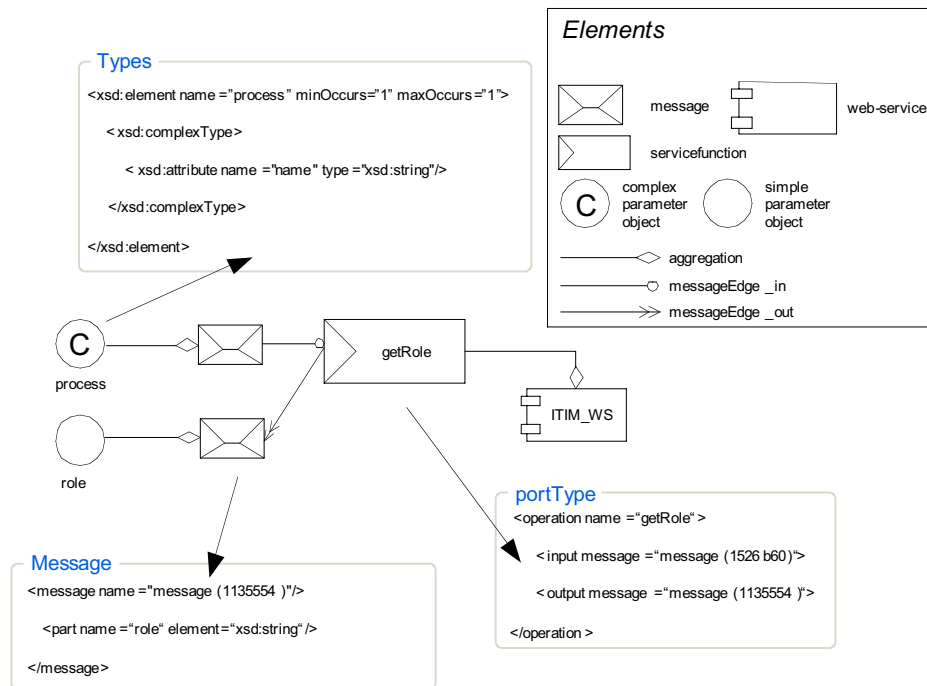
Figure 3. Web-service modeling language
