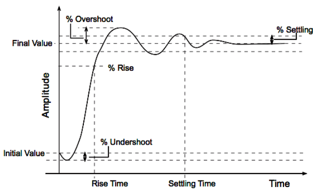
Fig. 2 Signal Constraints for a unit step input
