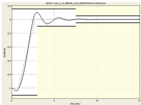
Fig. 4 Pre-Optimization Response
