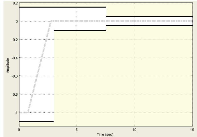
Fig. 3 u_{ref} and Constraints in Simulink SCB
