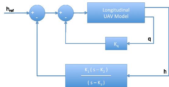
Fig. 1 Altitude-Acquire & Hold Phase Lead Compensator
