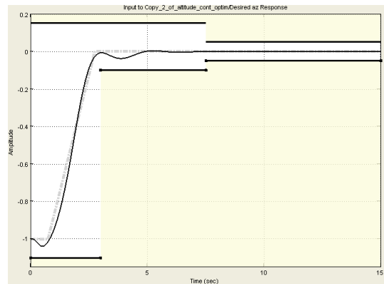
Fig. 5 Optimized Solution
