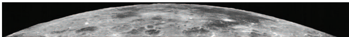
FIGURE 1 Densely cratered part of the surface of the Moon (APOLLO 17, PHOTO P-2871)
