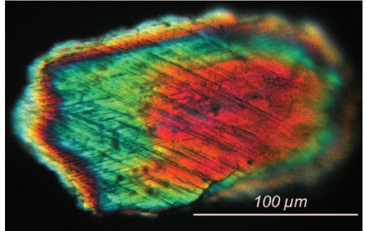
FIGURE 3 Shocked quartz grain from ejecta of the Manson crater (USA), demonstrating the characteristic “planar deformation features” (PDFs). These features are straight, penetrate the whole crystal, and occur in more than one orientation. Wavy lamellae, observed in some quartz grains, are not characteristic of shock. Micrograph between crossed polarizers.
