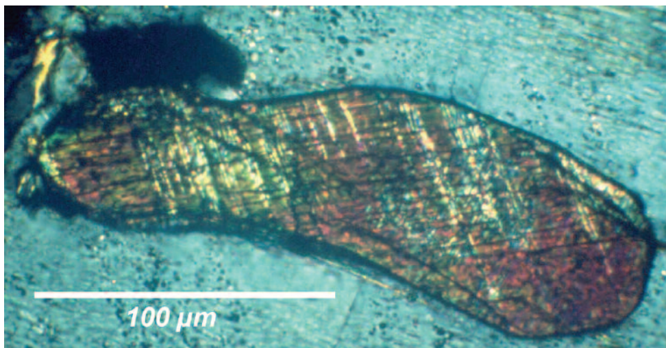
FIGURE 7 Shocked zircon grain from the Vredefort structure, South Africa. Micrograph between crossed polarizers. PHOTO COURTESY R. GIBSON AND U. REIMOLD
