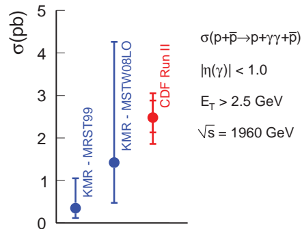
FIG. 4. Comparison of the measured cross section for the exclusive \gamma\gamma production in p\bar{p} collisions at \sqrt{s} = 1.96 \text{ TeV} with theoretical predictions [9].
