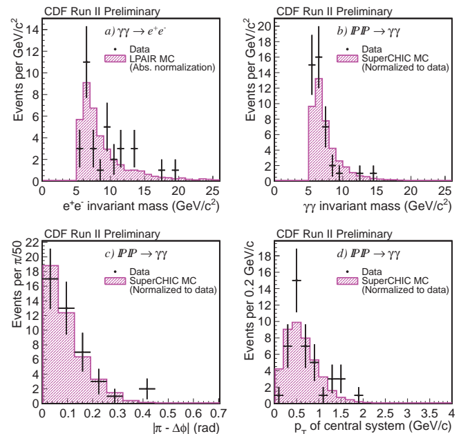
FIG. 2. The e^+e^- candidates: invariant mass distribution (a). The two-photon candidates: invariant mass distribution (b), |\pi - \Delta\phi| distribution (c), and p_T distribution of the two photons. All error bars are statistical. The MC predictions for \gamma\gamma are normalized to data. The QED prediction for e^+e^- is normalized to the delivered luminosity and efficiencies.
