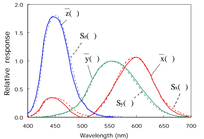
Figure 2. Spectral responsivities of Colorimeter 1.
