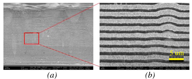
Fig. 4: SEM images of the side views of the Zn anode before discharge test: (a) sidewall of the 50-layer skeleton structure after Zn electroplating, (b) enlarged image showing the 1.4 μm thick Zn coated layers.
