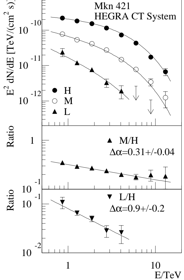
Fig. 3. For three distinct flux intervals (H,M,L, see Table 2), the energy spectra have been extracted and the flux ratios calculated. The energy spectra get considerably softer with decreasing average flux. The cut-off energy remains unchanged within the statistical error.
