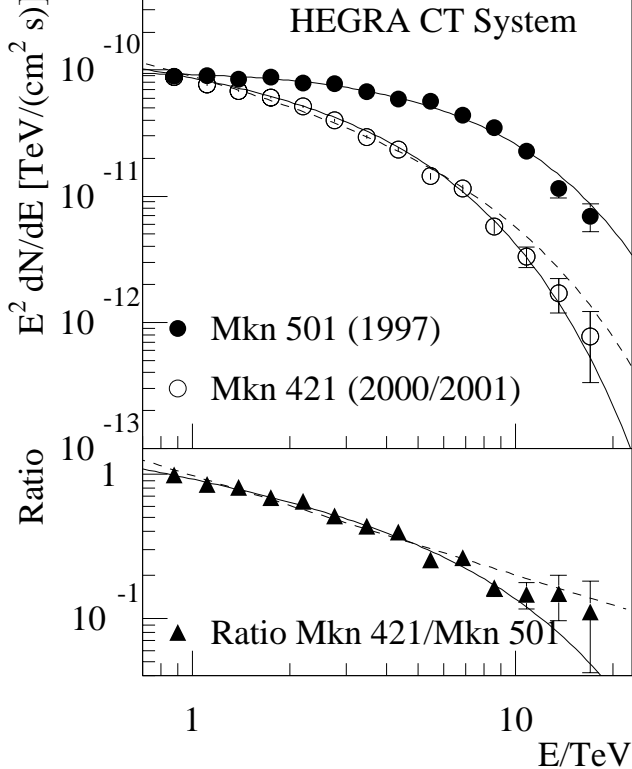
Fig. 9. Comparing the energy spectra of Mkn 501 (Aharonian et al., 1999a) with the measurements of Mkn 421 (2000/2001): The observed differential spectra are well described by a power law with exponential cut-off (see Eqn. 1). Both, the cut-off energy and the photon index differ for the two energy spectra ( \alpha_{Mkn501} = 1.92 \pm 0.03_{\text{stat}} \pm 0.2_{\text{sys}} , \alpha_{Mkn421} = 2.19 \pm 0.02_{\text{stat}} \pm 0.04_{\text{sys}} ). A fit of a fixed cut-off energy at 6.2 TeV as measured for Mkn 501 while letting the photon index vary to the Mkn 421 data results in the dashed curve in the upper panel with \chi^2_{\text{red}} = 5.7(12) , excluding the larger cut-off energy provided that systematic effects are negligible. To further study the difference of the energy spectra and to reduce the impact of possible systematic effects, the ratio of the two energy spectra are calculated. The flux ratio is not compatible with a pure power law model (dashed curve, \chi^2_{\text{red}} = 3.6(12) ) indicating a difference in the shape of the two energy spectra. A function of the form given in Eqn 2 gives an acceptable fit ( \chi^2_{\text{red}}(d.o.f.) = 1.5(12) ) with \Delta\alpha = 0.35 \pm 0.07 and c = (0.12 \pm 0.02) \text{ TeV}^{-1} .
