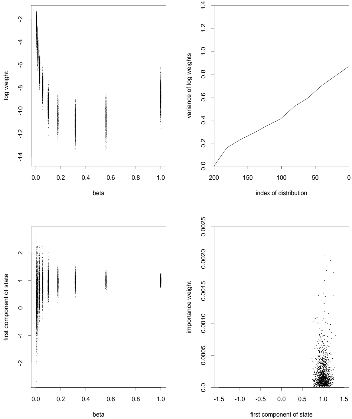
Figure 1: Results of the first test on the unimodal distribution. Upper left: the logs of the importance weights at ten values of \beta , for each of the 1000 runs. Upper right: the variance of the log weights as a function of the index of \beta . Lower left: the distribution of the first component of the state at ten \beta values. Lower right: the joint distribution of the first component and the importance weight at the ends of the runs. Random jitter was added to the \beta values in the plots on the left to improve the presentation.
