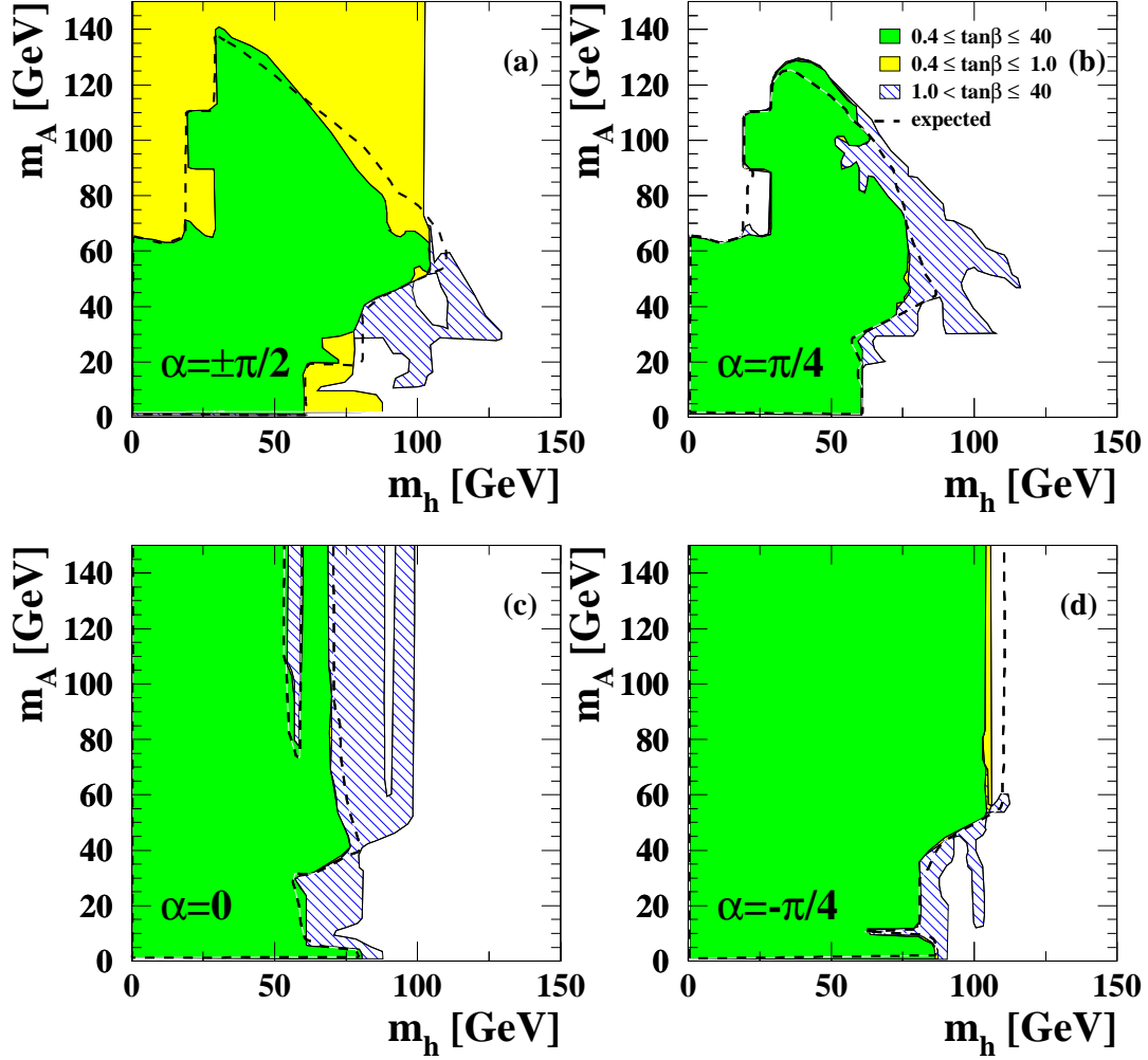
Figure 7: Excluded regions in the (m_h, m_A) plane, (a)–(d), for \alpha = \pm\pi/2 , \pi/4 , 0 and -\pi/4 , respectively, together with the expected exclusion limits. A particular (m_h, m_A, \alpha) point is excluded at 95% CL if it is excluded for all scanned values of \tan\beta . Three different domains of \tan\beta are shown: the darker grey region is excluded for all values 0.4 \leq \tan\beta \leq 40 ; additional enlarged excluded regions are obtained constraining 0.4 \leq \tan\beta \leq 1.0 (lighter grey area) or 1.0 < \tan\beta \leq 40 (hatched area). Expected exclusion limits for 0.4 \leq \tan\beta \leq 40 are shown as a dashed line.
