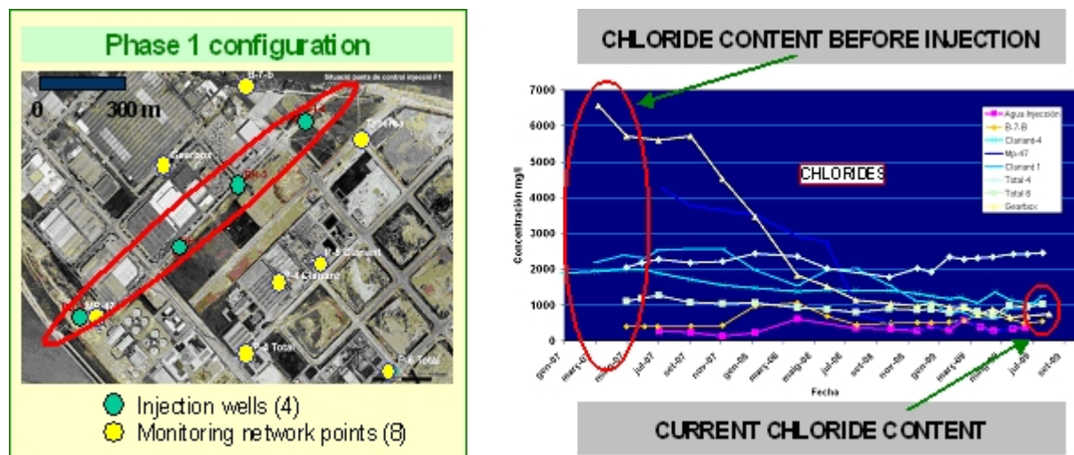
Figure 2: Pilot phase configuration of the hydraulic barrier project and chloride evolution in the monitoring control points between January 2007 and September 2009. Water injection started March 2007.
