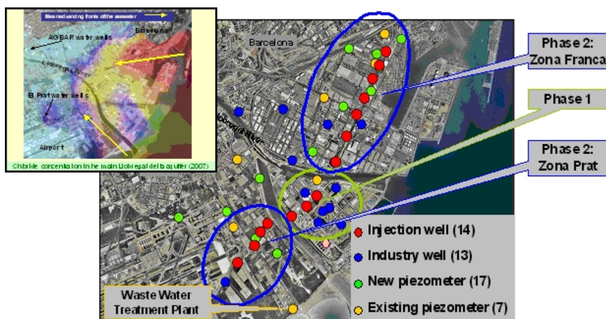
Figure 1: Chloride concentration in the main Llobregat delta aquifer (2007) and hydraulic barrier network configuration (injection wells and monitoring points). The project has been performed in two phases.
