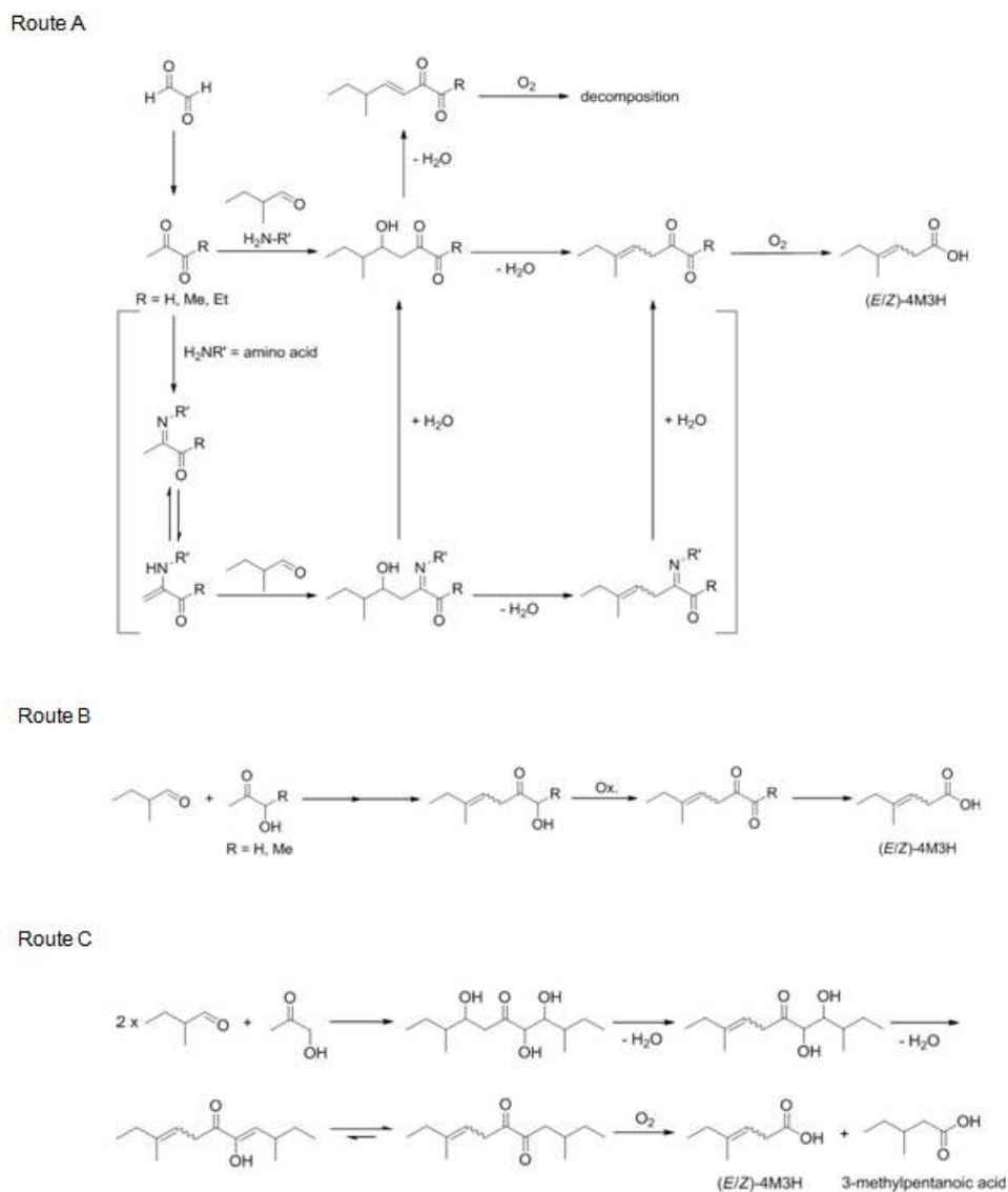
Fig. 4: The proposed formation pathways of 4-methyl-3-hexenoic acid (4M3H) in the model maillard reactions of L-isoleucine with sugars, starting from 2-methylbutanal and the sugar degradation compounds (glyoxal, 2-oxopropanal, 2, 3-butanedione, 2, 3-pentanedione, 1-hydroxy-2-propanone and 3-hydroxy-2-butanone)
