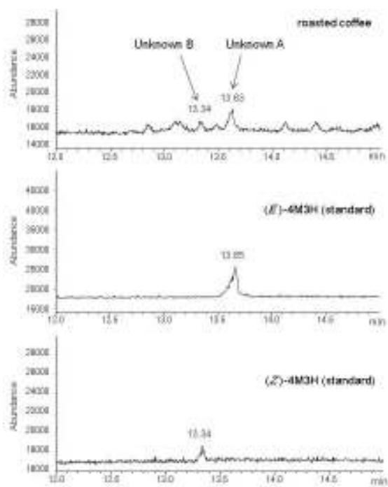
Fig. 1: The total ion chromatogram of 4-methyl-3-hexenoic acid (4M3H) found in roasted coffee, via Multidimensional Gas Chromatography-Mass Spectrometry (MDGC-MS) (column (second dimension), InertCap1; ( E )-4M3H, 13.65 min; ( Z )-4M3H, 13.34 min)
