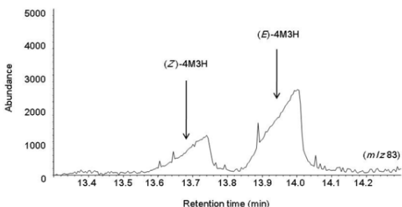
Fig. 3: The extracted ion chromatogram of 4-methyl-3-hexenoic acid (4M3H) formed in the maillard reaction of L-isoleucine with xylose, via Multidimensional Gas Chromatography-Mass Spectrometry (MDGC-MS) (selected ion, m/z 83; column (second dimension), InertCap 1)
